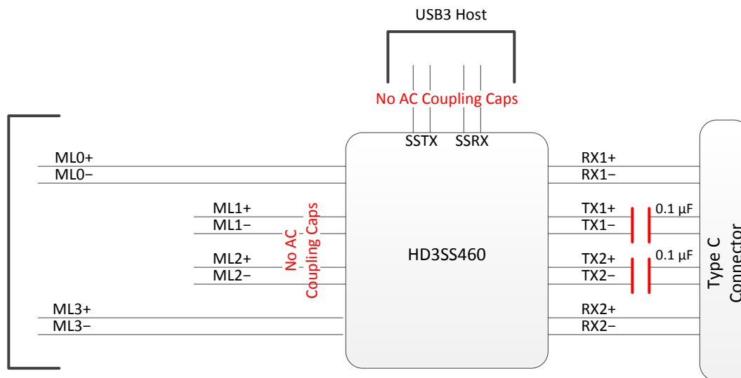
Figure 4. HD3SS460 USB Host/DP Source Implementation Example With 0\text{ V} < \text{SSTX/RX } V_{cm} < 2\text{ V}
