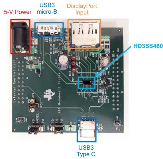
Figure 1. HD3SS460EVM-SRC
