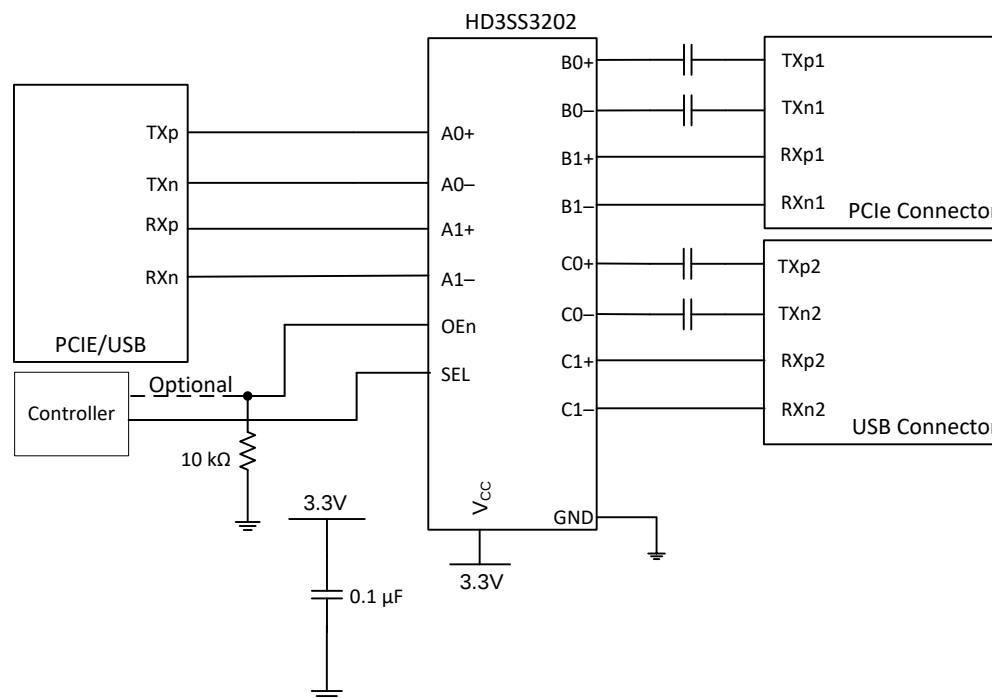
Figure 13. PCIE Motherboard
