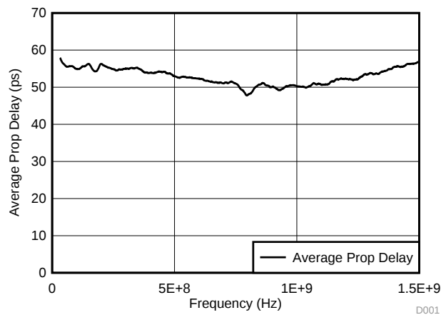
Figure 1. Average Propagation Delay vs Frequency
