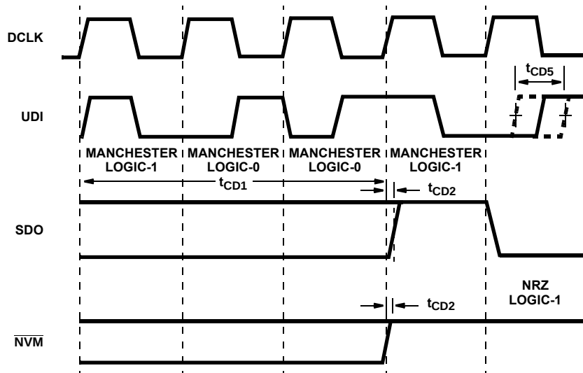
FIGURE 12. ENCODER TIMING
