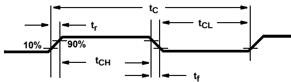
FIGURE 9. CLOCK TIMING
