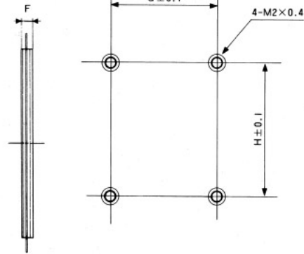
PCB Mounting Pattern
