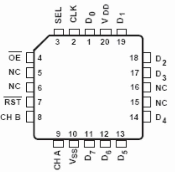
PINOUT C
