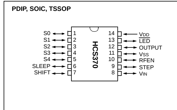
FIGURE 1-1: HCS370 DIAGRAM
