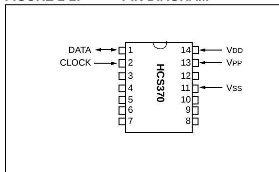
FIGURE 1-2: PIN DIAGRAM
