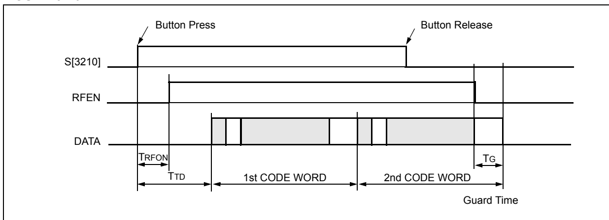
FIGURE 3-10: PLL INTERFACE
