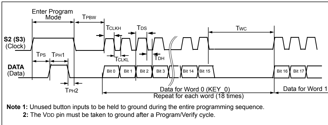
FIGURE 5-1: PROGRAMMING WAVEFORMS
