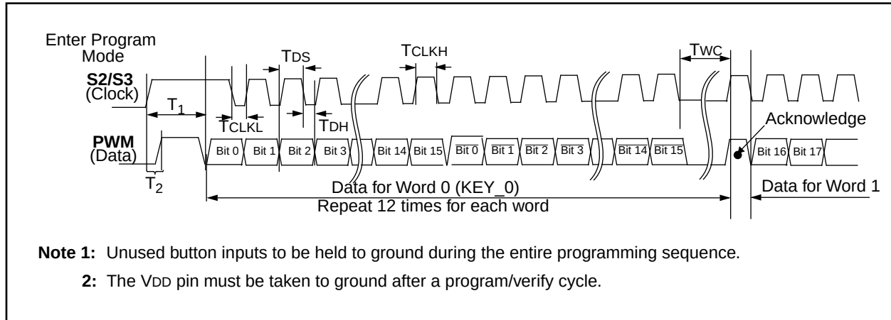
FIGURE 6-1: PROGRAMMING WAVEFORMS
