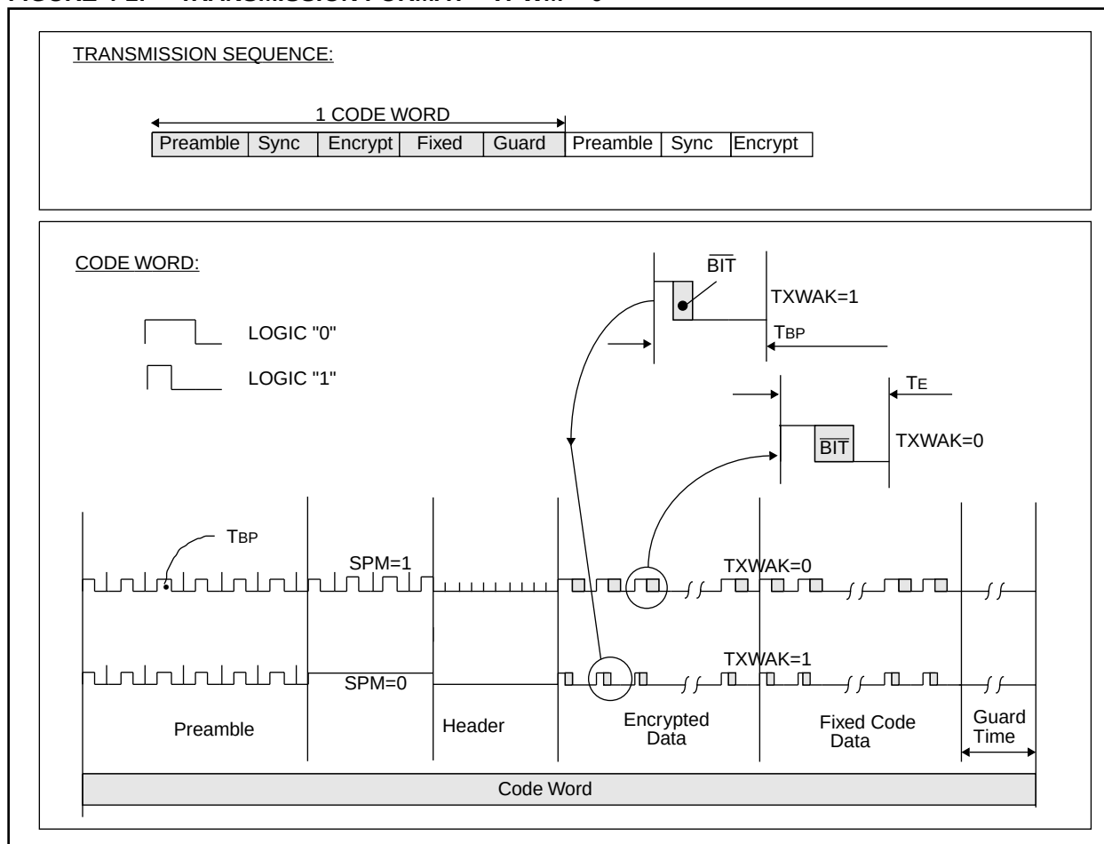
FIGURE 4-1: TRANSMISSION FORMAT—VPWM = 0
