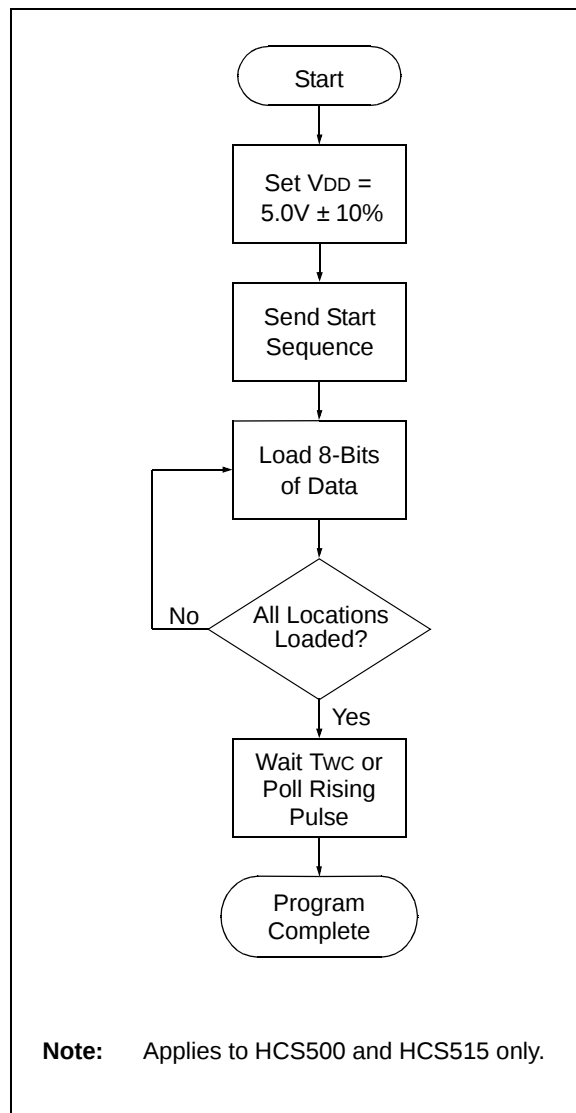
FIGURE 4-7: PROGRAMMING FLOW CHART 4
