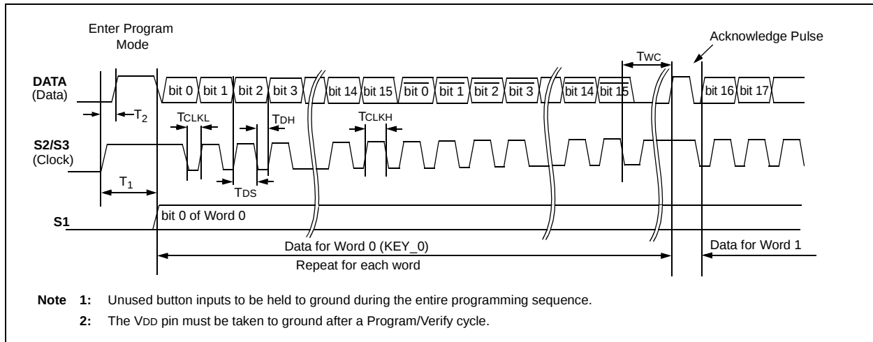
FIGURE 5-5: PROGRAMMING WAVEFORMS
