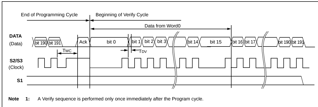
FIGURE 5-6: VERIFY WAVEFORMS
