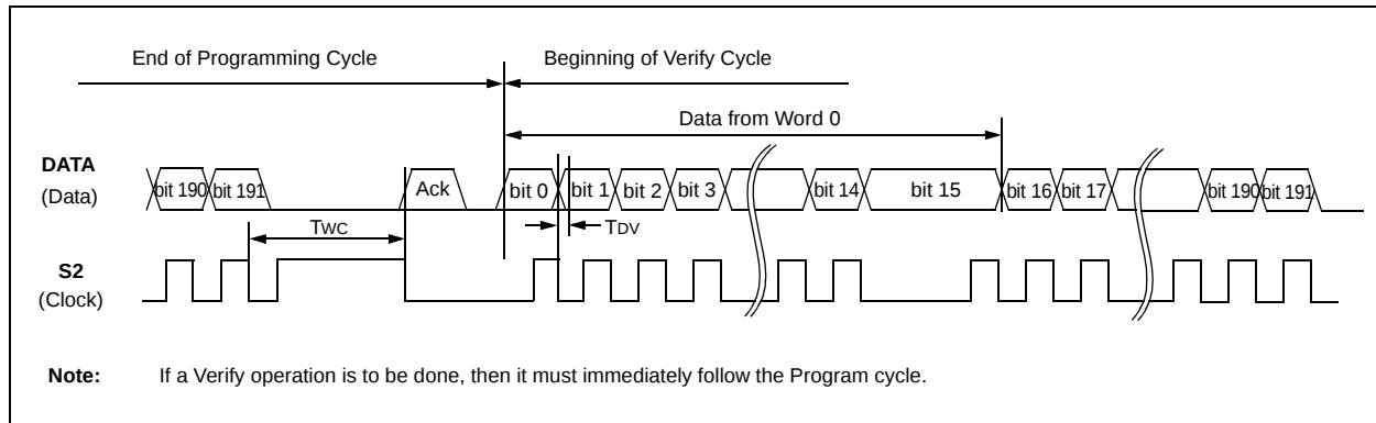
FIGURE 5-4: VERIFY WAVEFORMS
