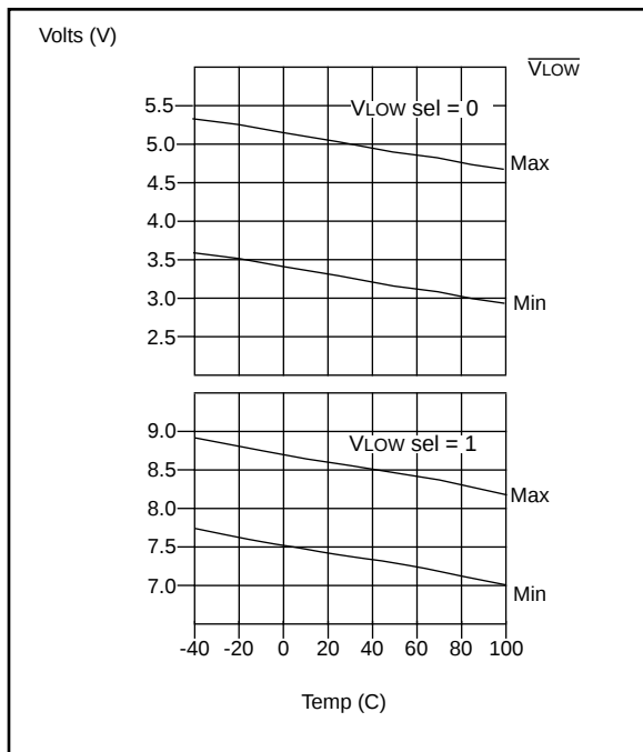
FIGURE 3-1: VOLTAGE TRIP POINTS BY CHARACTERIZATION
