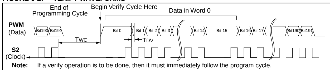
FIGURE 6-2: VERIFY WAVEFORMS
