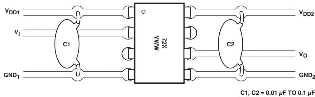
Figure 11. Recommended printed circuit board layout
