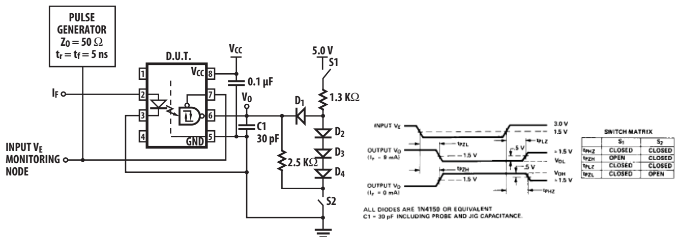
Figure 8. Test circuit for t_{PHZ} , t_{PZH} , t_{PLZ} , and t_{PLH} (single channel product only)
