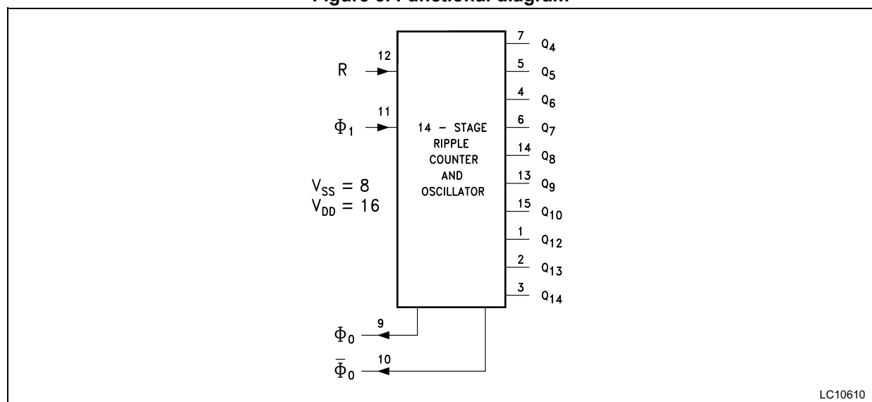
Figure 3. Functional diagram
