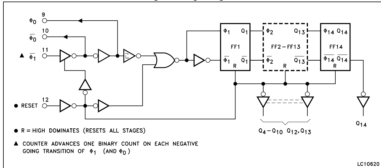
Figure 3. Functional diagram
