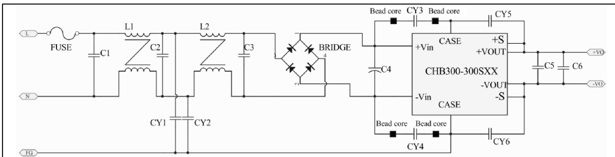
Circuit Connection
