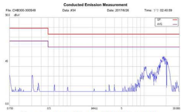
Class A conducted Test for HB300S48-6.25 Line
