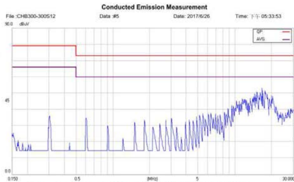
Class A conducted Test for HB300S12-25 Nature
