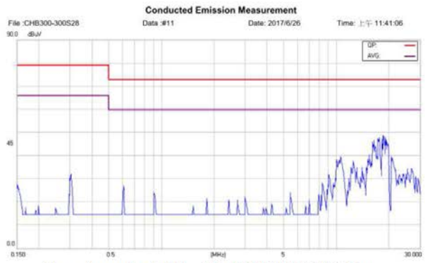
Class A conducted Test for HB300S28-10.7 Line
