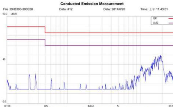
Class A conducted Test for HB300S28-10.7 Nature
