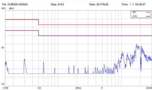
Class A conducted Test for HB300S24-12.5 Line
