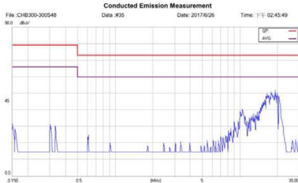
Class A conducted Test for HB300S48-6.25 Nature
