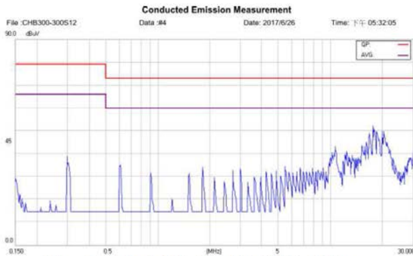
Class A conducted Test for HB300S12-25 Line
