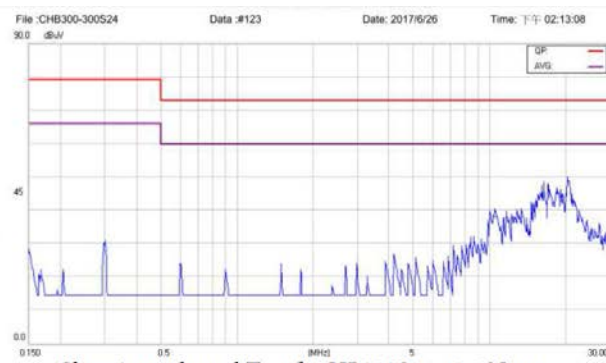
Class A conducted Test for HB300S24-12.5 Nature
