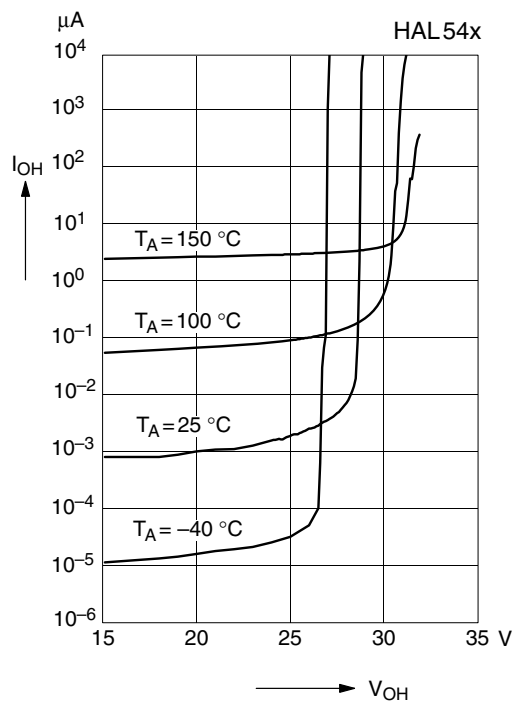
Fig. 3-15: Typ. output high current versus output voltage
