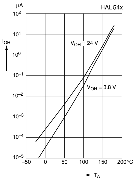
Fig. 3-16: Typical output leakage current versus ambient temperature
