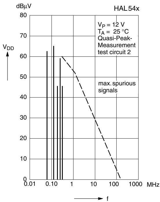
Fig. 3-18: Typ. spectrum of supply voltage
