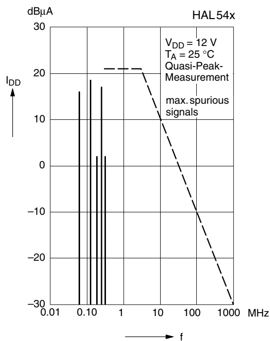
Fig. 3-17: Typ. spectrum of supply current
