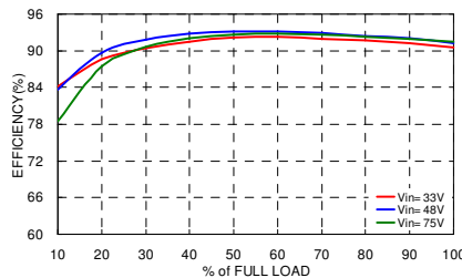
HAE200-48S05 Efficiency vs. Output Load
