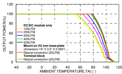
HAE150-48S05 Derating Curve
