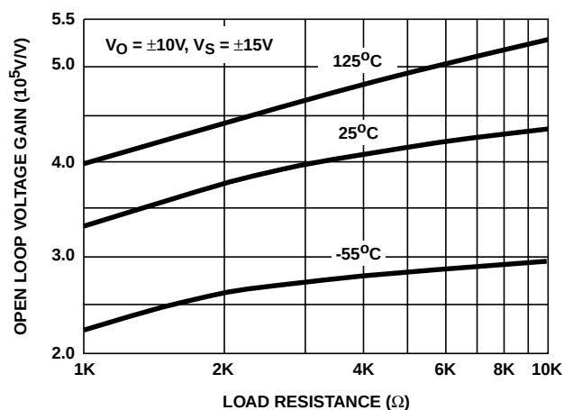
FIGURE 16. A_{VOL} vs LOAD RESISTANCE
