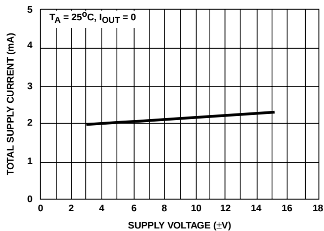
FIGURE 14. I_{CC} vs V_S (HA-5102)
