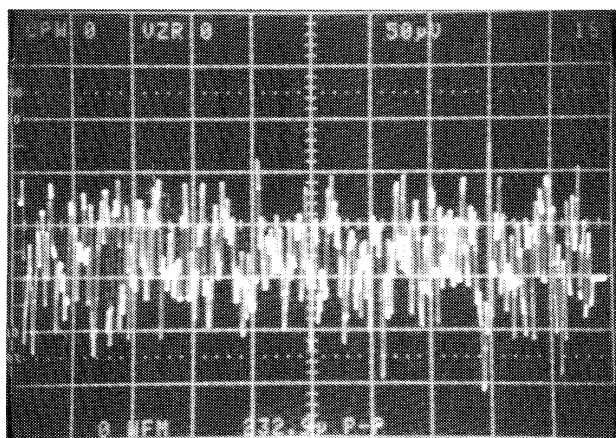
FIGURE 5. INPUT NOISE VOLTAGE DENSITY
