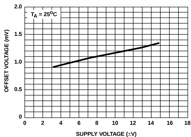
FIGURE 10. V_{IO} vs V_S
