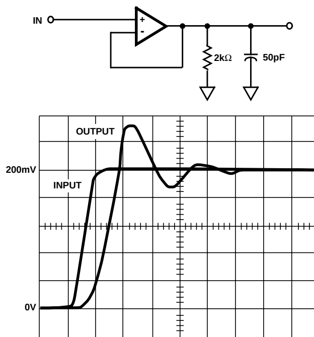
FIGURE 2. SMALL SIGNAL RESPONSE CIRCUIT
