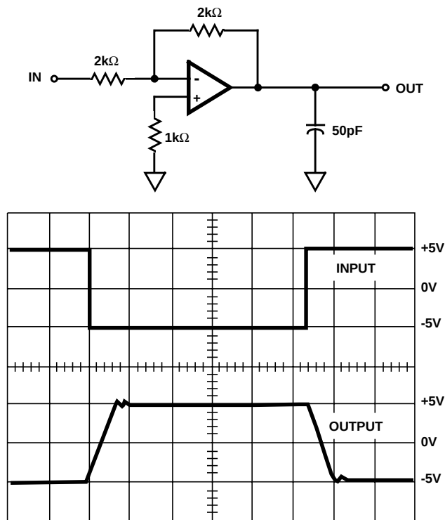
FIGURE 1. LARGE SIGNAL RESPONSE CIRCUIT
