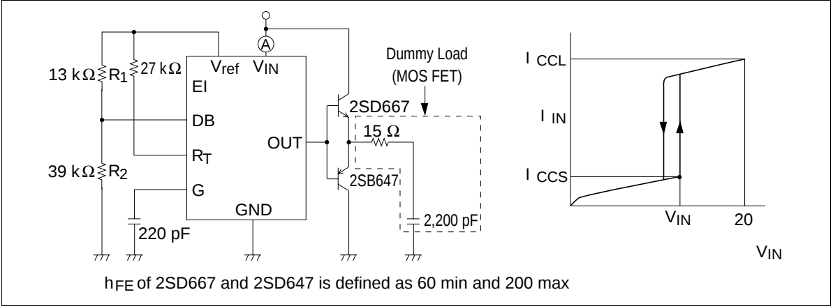
Figure 2 I CCS • I CCL Measurement Circuit
