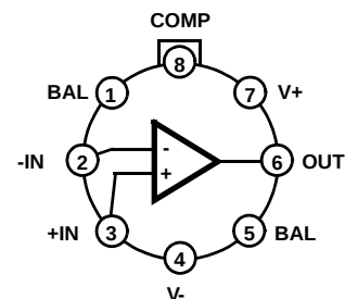
HA-2620 (METAL CAN) TOP VIEW
