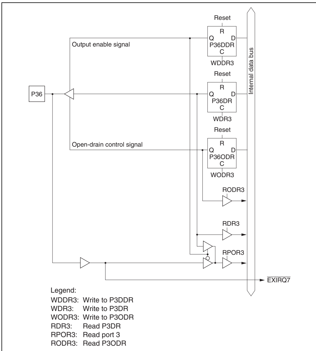
Figure C.8 Port 3 Block Diagram (Pin P36)
