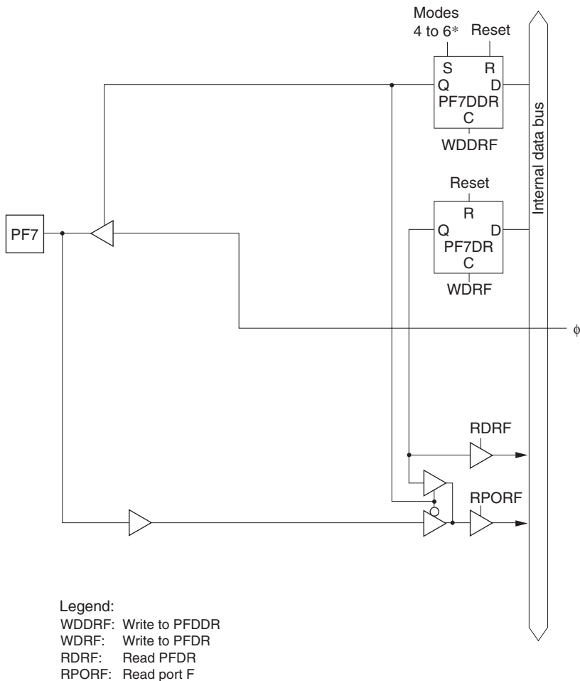
Figure C.30 Port F Block Diagram (Pin PF7)
