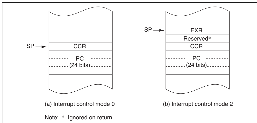
Figure 4.6 Stack Status after Exception Handling (Advanced Modes)
