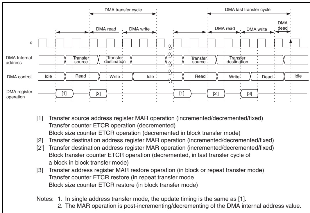
Figure 7.29 DMAC Register Update Timing
