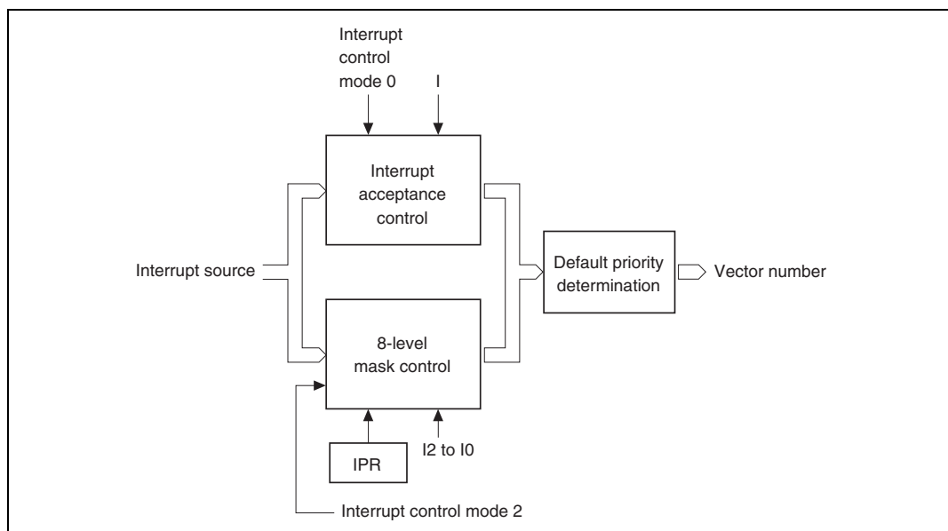
Figure 5.4 Block Diagram of Interrupt Control Operation
