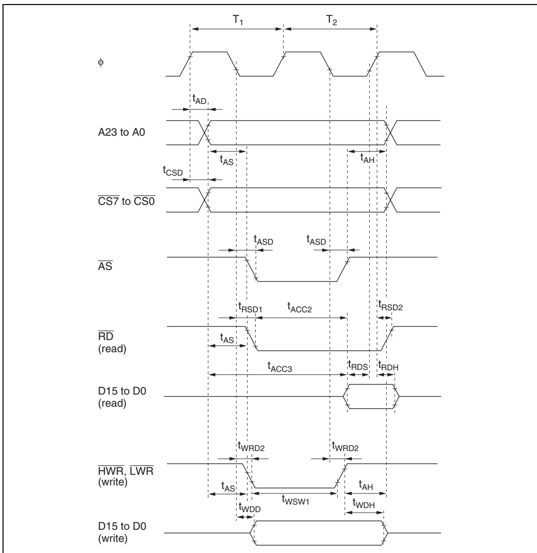
Figure 18.7 Basic Bus Timing/Two-State Access
