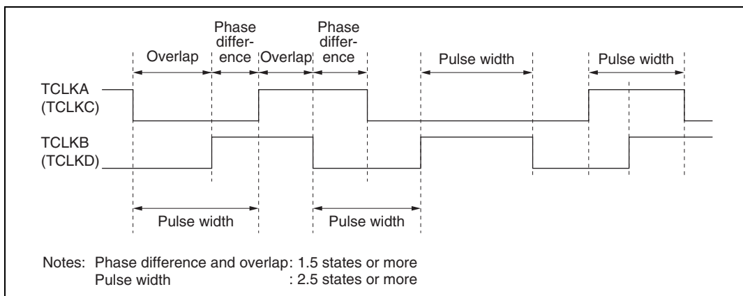
Figure 10.44 Phase Difference, Overlap, and Pulse Width in Phase Counting Mode
