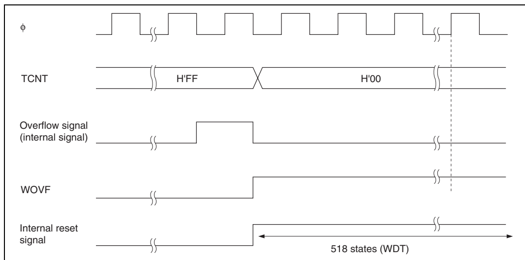
Figure 11.7 Timing of WOVSF Setting
