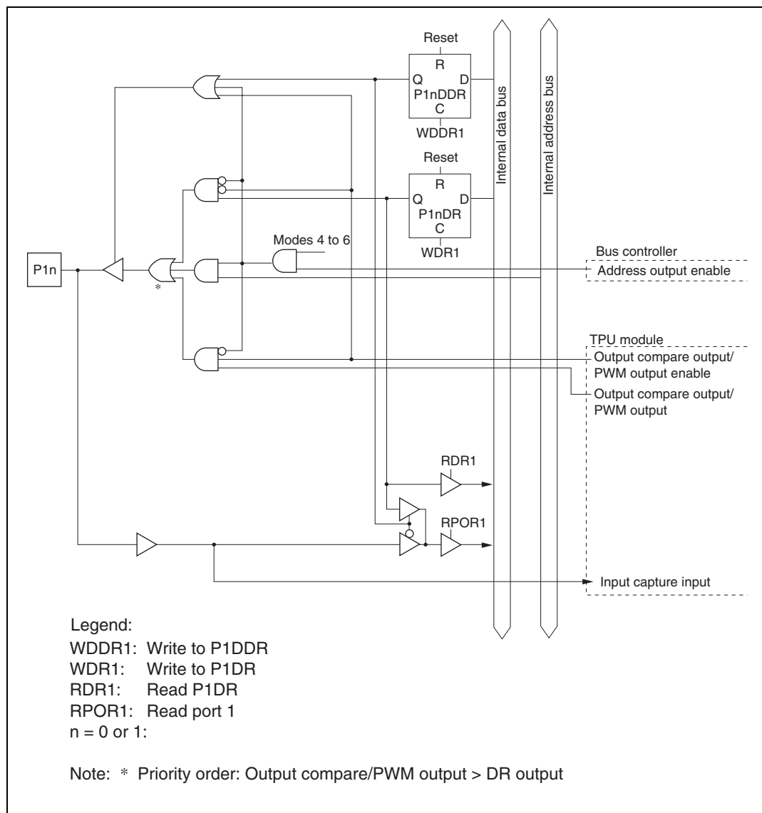
Figure C.1 Port 1 Block Diagram (Pins P10 and P11)
