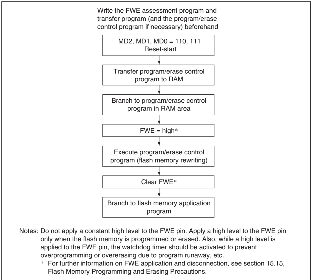
Figure 15.13 User Program Mode Execution Procedure
