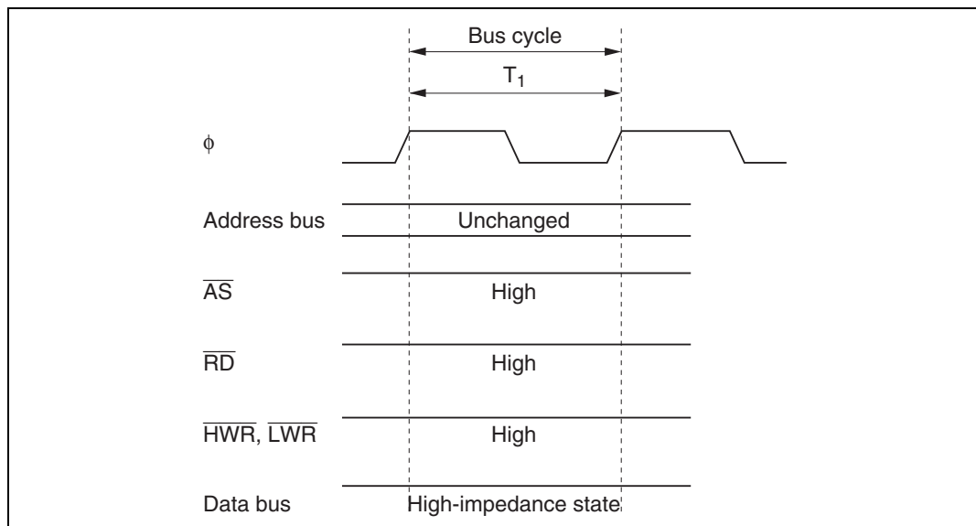
Figure 2.19 Pin States during On-Chip Memory Access
