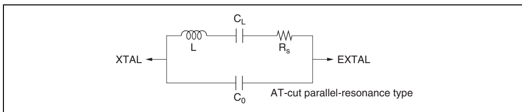
Figure 16.3 Crystal Resonator Equivalent Circuit
