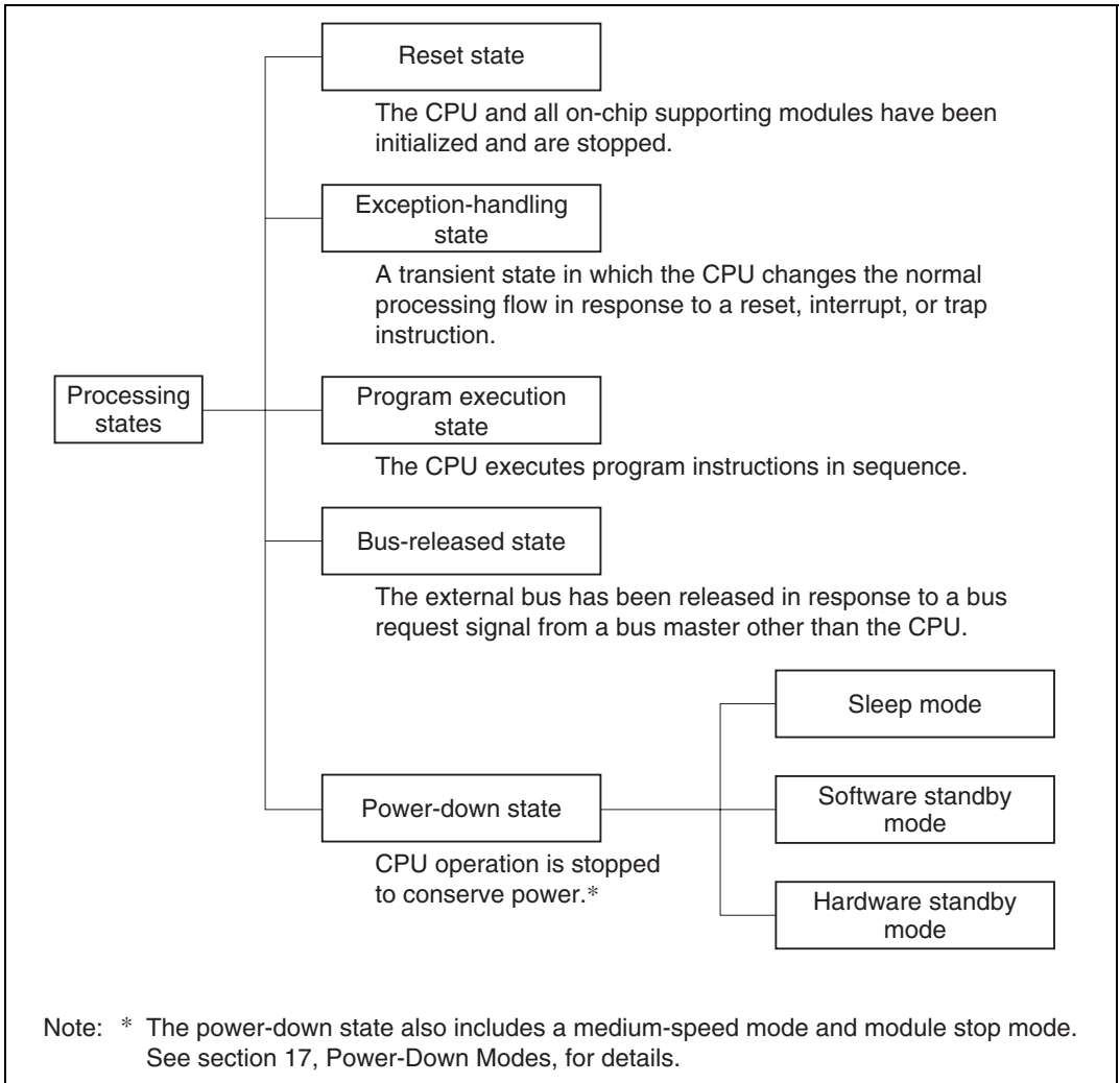
Figure 2.15 Processing States
