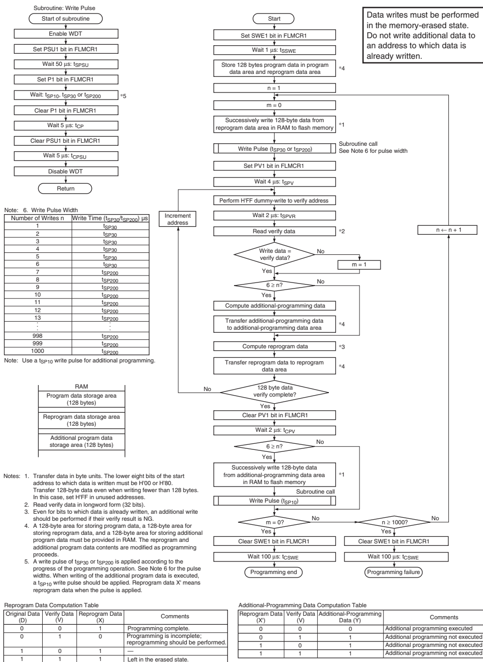
Figure 15.14 Program/Program-Verify Flowchart
