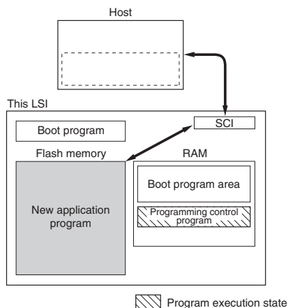
Figure 15.4 Boot Mode
