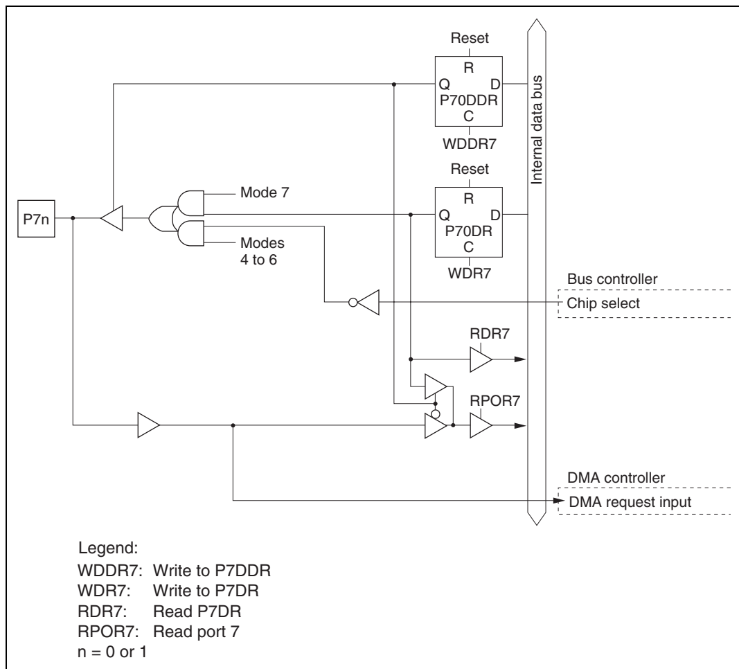
Figure C.11 Port 7 Block Diagram (Pins P70 and P71)
