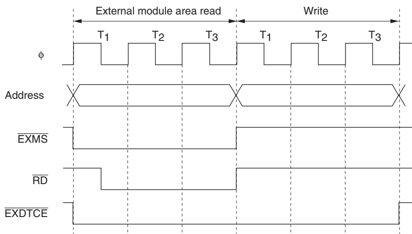
(a) Timing of external module area read by DTC
