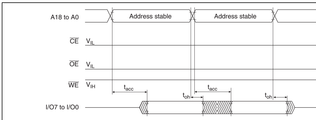
Figure 15.23 \overline{\text{CE}} and \overline{\text{OE}} Enable State Read Timing Waveforms
