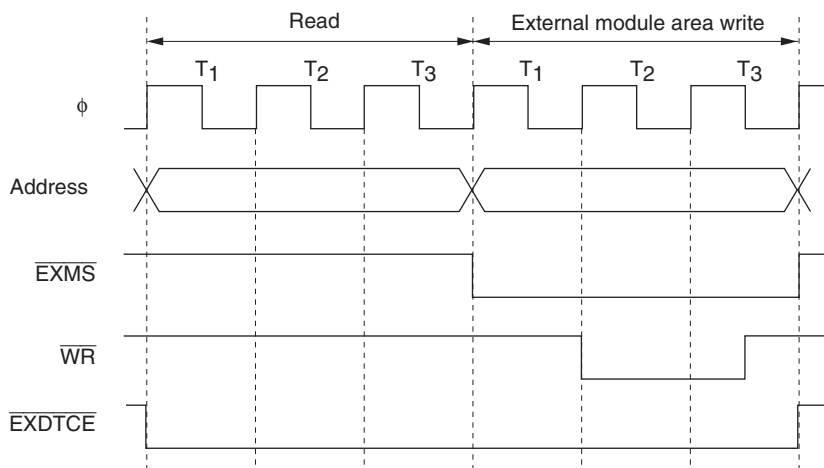
(b) Timing of external module area write by DTC
