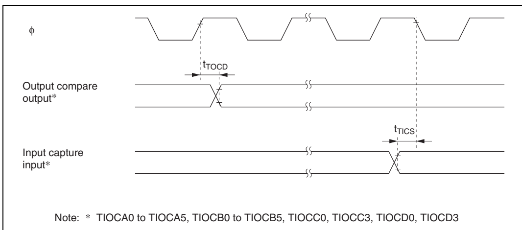
Figure 18.13 TPU Input/Output Timing
