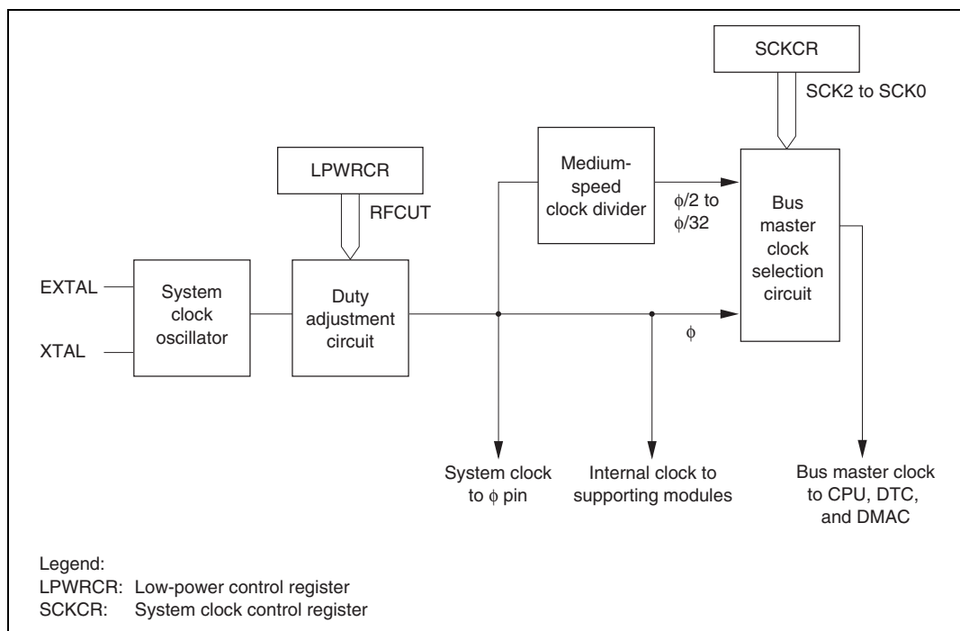
Figure 16.1 Block Diagram of Clock Pulse Generator
