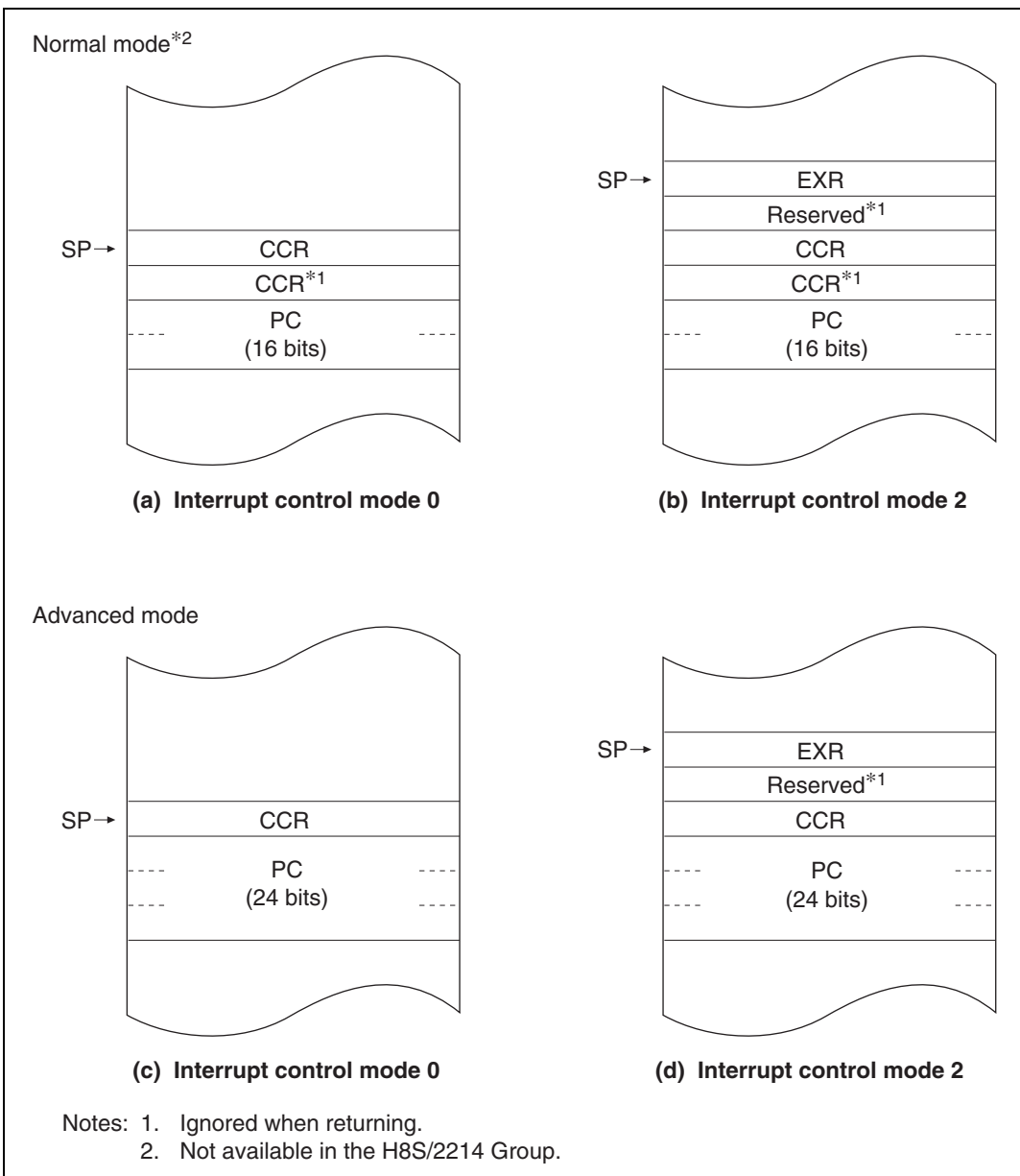
Figure 2.17 Stack Structure after Exception Handling (Examples)
