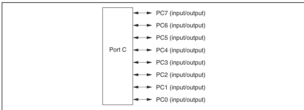
Figure 9.11 Port C Pin Functions (Mode 7)
