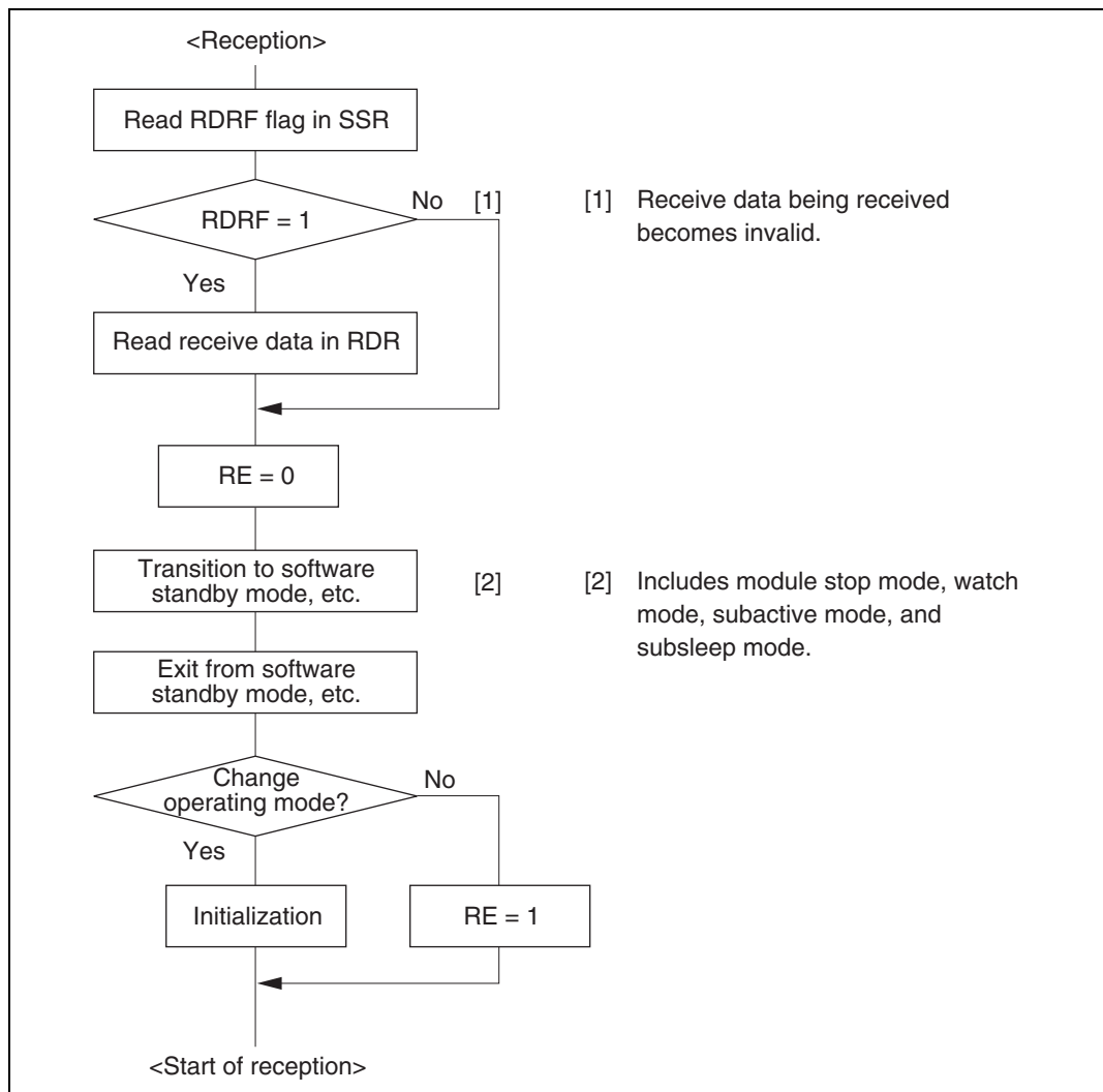
Figure 12.31 Sample Flowchart for Mode Transition during Reception
