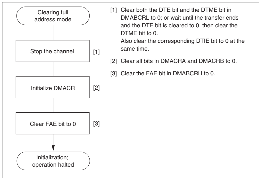
Figure 7.27 Example of Procedure for Clearing Full Address Mode
