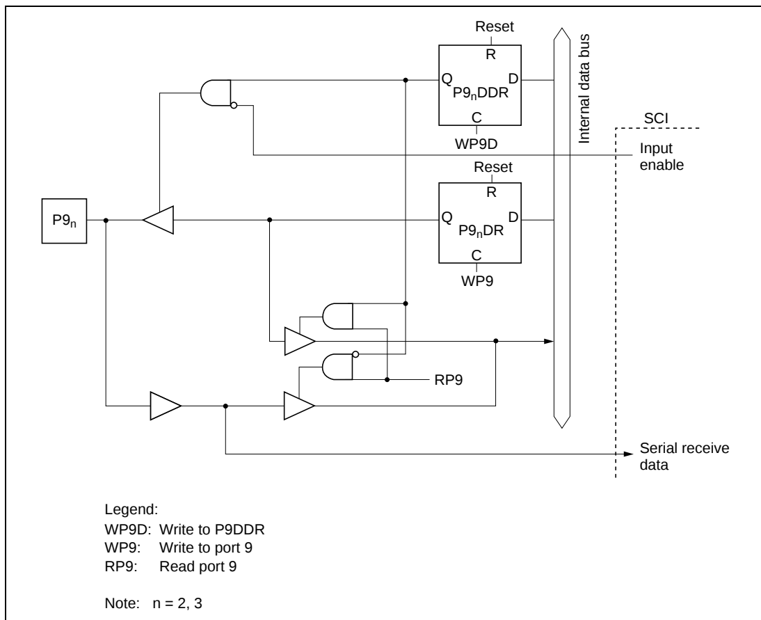
Figure C.8 (c) Port 9 Block Diagram (Pin P9 2 , P9 3 )
