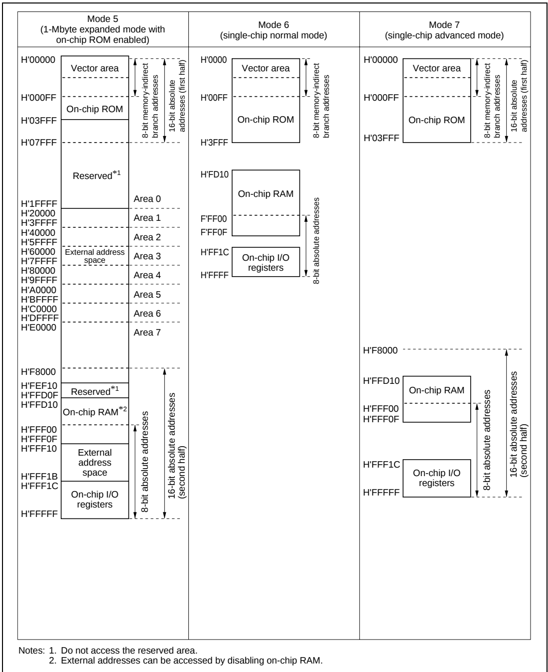
Figure 3.4 H8/3036 Memory Map in Each Operating Mode (2)
