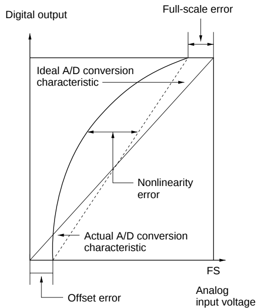
Figure 13.10 A/D Conversion Precision Definitions (2)
