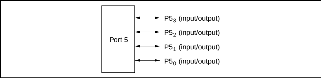
Figure 7.15 Pin Functions in Mode 6 and 7 (Port 5)
