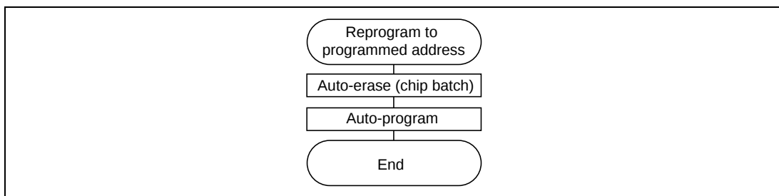
Figure 15.24 Reprogramming to Programmed Address
