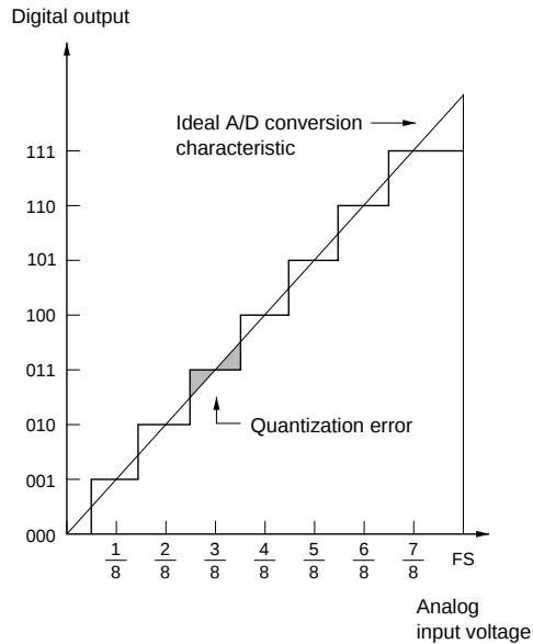
Figure 13.9 A/D Conversion Precision Definitions (1)
