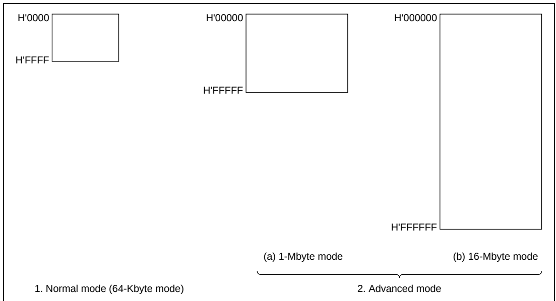
Figure 2.2 Memory Map
