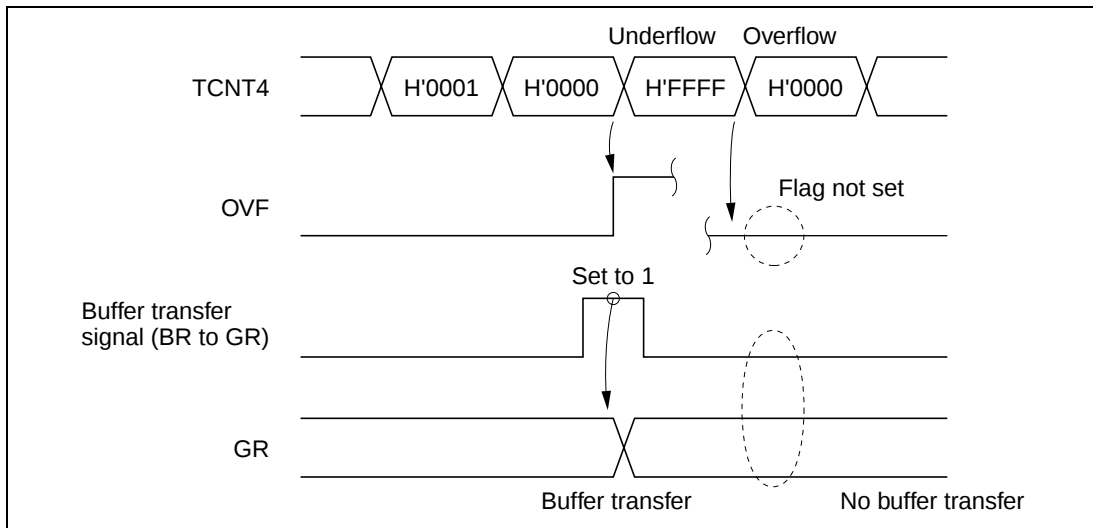
Figure 8.38 Undershoot Timing
