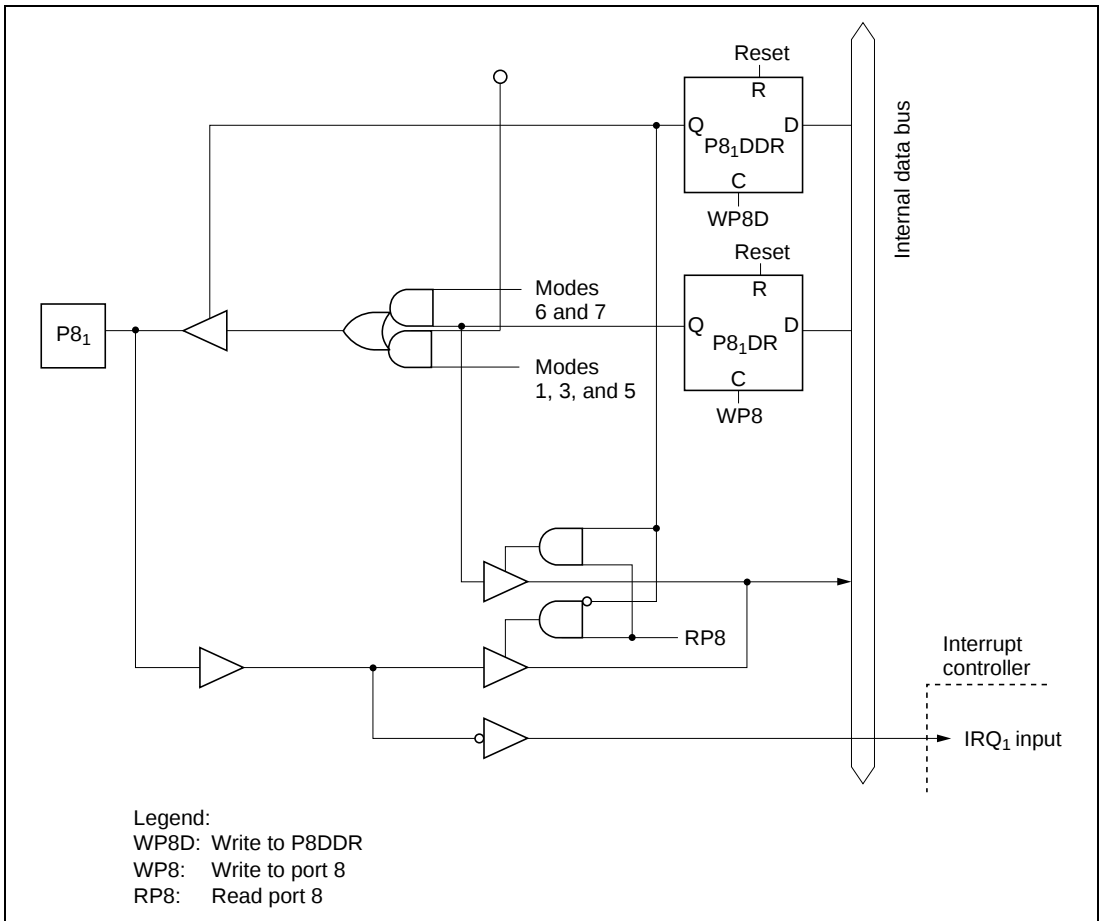
Figure C.7 (b) Port 8 Block Diagram (Pin P8 i )
