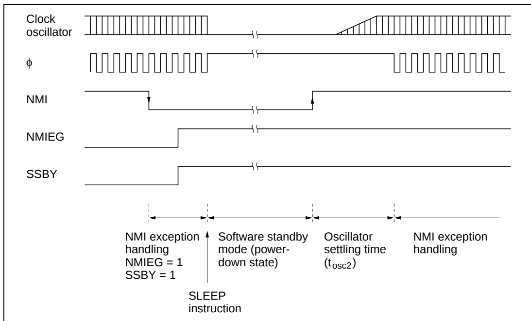
Figure 17.1 NMI Timing for Software Standby Mode (Example)
