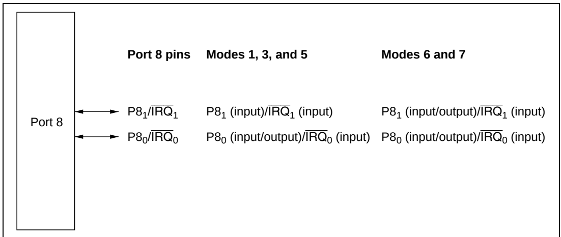
Figure 7.20 Port 8 Pin Configuration
