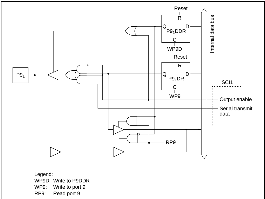
Figure C.8 (b) Port 9 Block Diagram (Pin P9 I )
