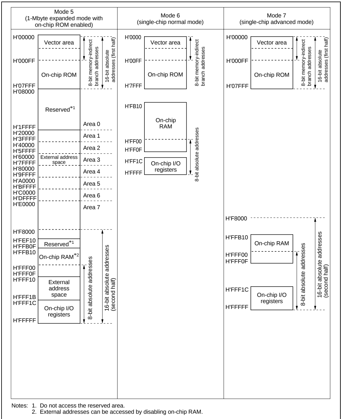
Figure 3.3 H8/3037 Memory Map in Each Operating Mode (2)
