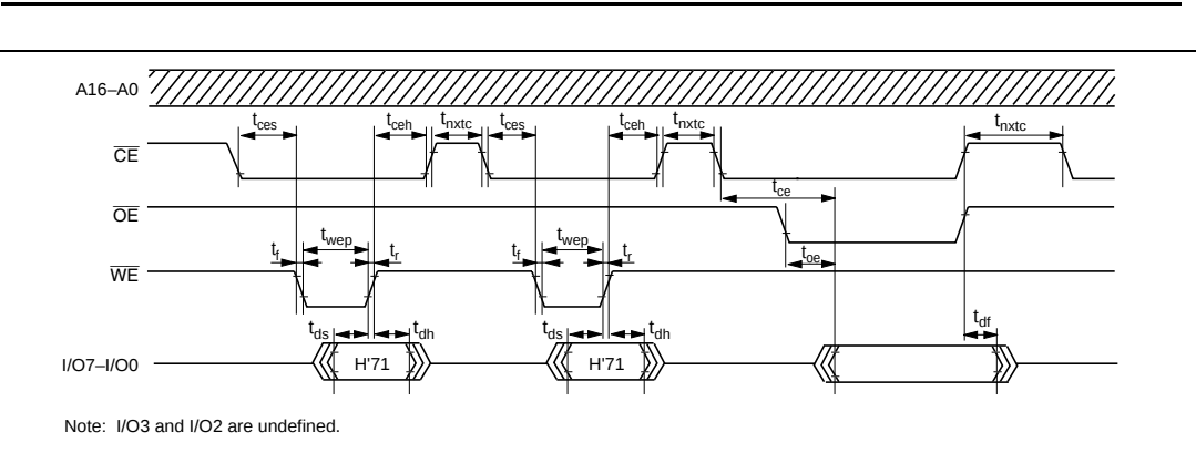
Figure 15.22 Status Read Mode Timing Waveforms
