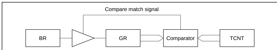
Figure 8.46 Compare Match Buffering
