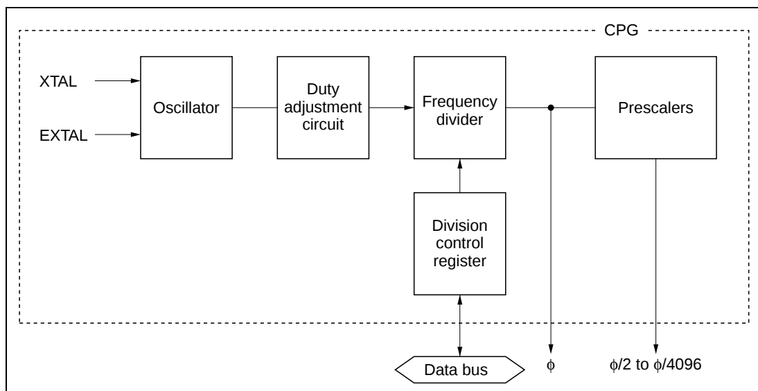
Figure 16.1 Block Diagram of Clock Pulse Generator
