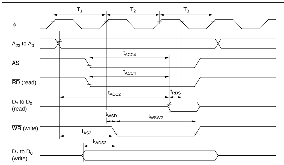
Figure 18.8 Basic Bus Cycle: Three-State Access
