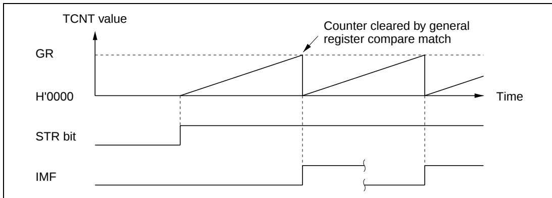
Figure 8.16 Periodic Counter Operation
