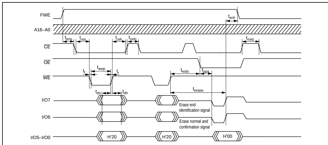
Figure 15.21 Auto-Erase Mode Timing Waveforms
