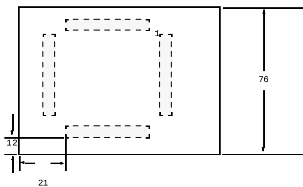
TOP VIEW (all dimensions in mm)
