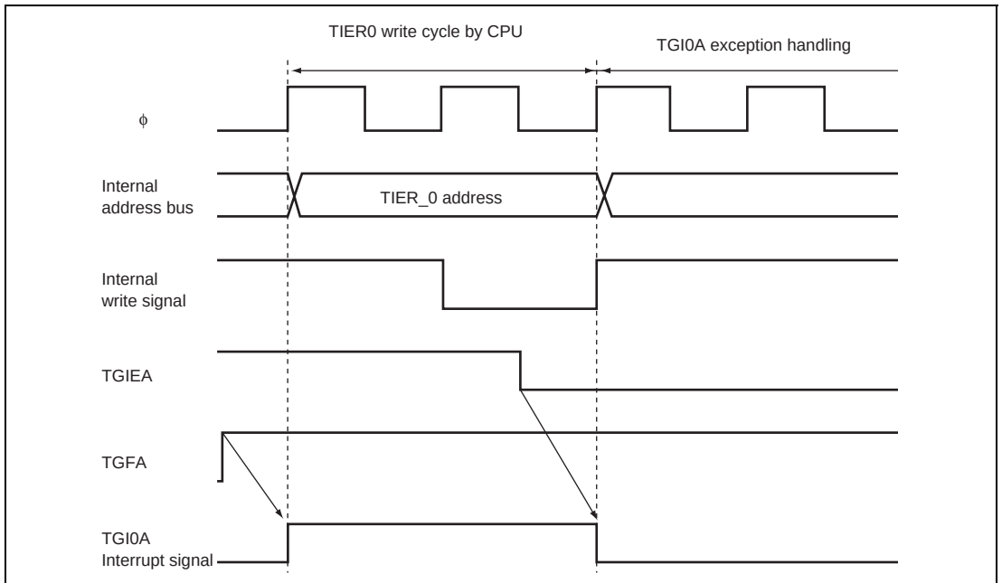
Figure 5.8 Contention between Interrupt Generation and Disabling
