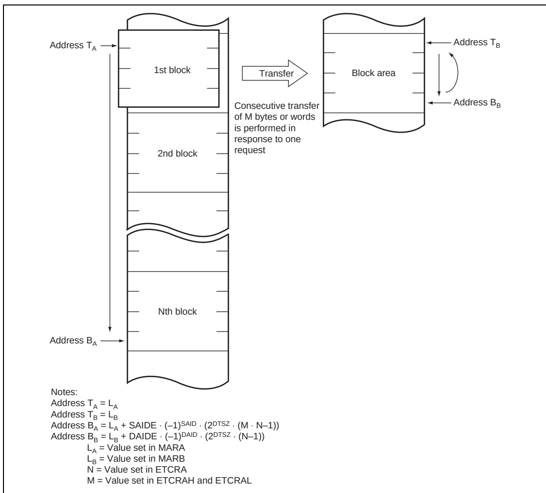
Figure 7.10 Operation in Block Transfer Mode (BLKDIR = 0)
