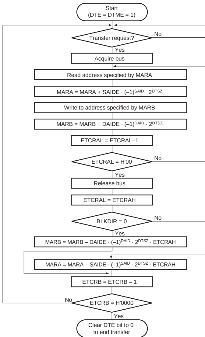
Figure 7.12 Operation Flow in Block Transfer Mode
