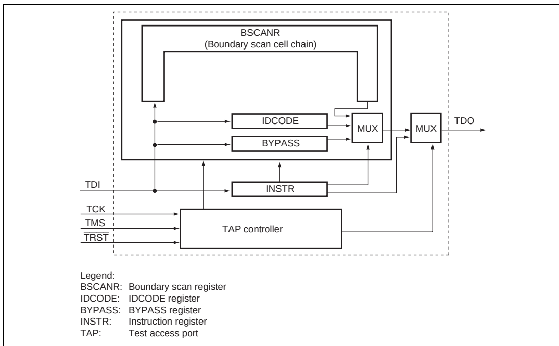
Figure 13.1 Block Diagram of Boundary Scan Function
