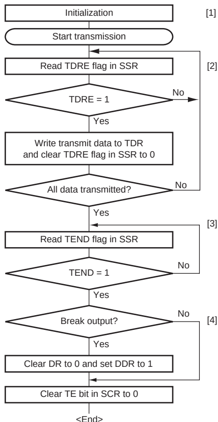
Figure 12.10 Sample Serial Data Transmission Flowchart
