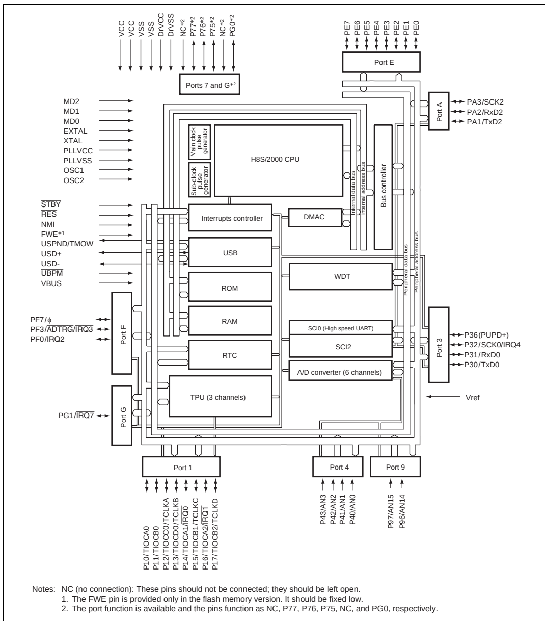
Figure 1.4 Internal Block Diagram of HD6432211, HD6432210 and HD6432210S
