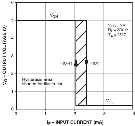
Figure 1. Transfer Characteristics
