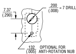
PANEL LAYOUT
