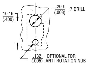
PANEL LAYOUT
