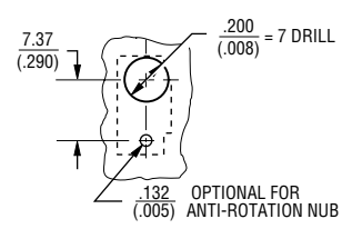
PANEL LAYOUT
