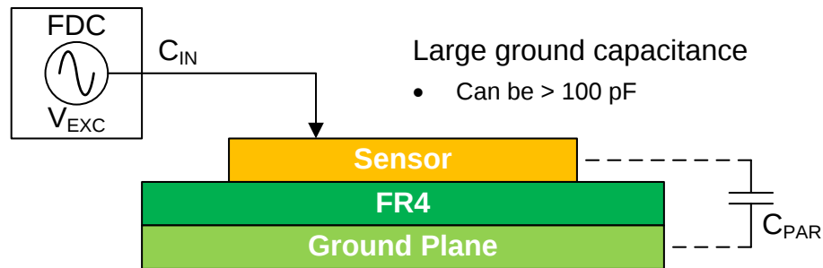
Figure 11. Ground Parasitic Capacitance Between the Ground Plane and the Sensor
