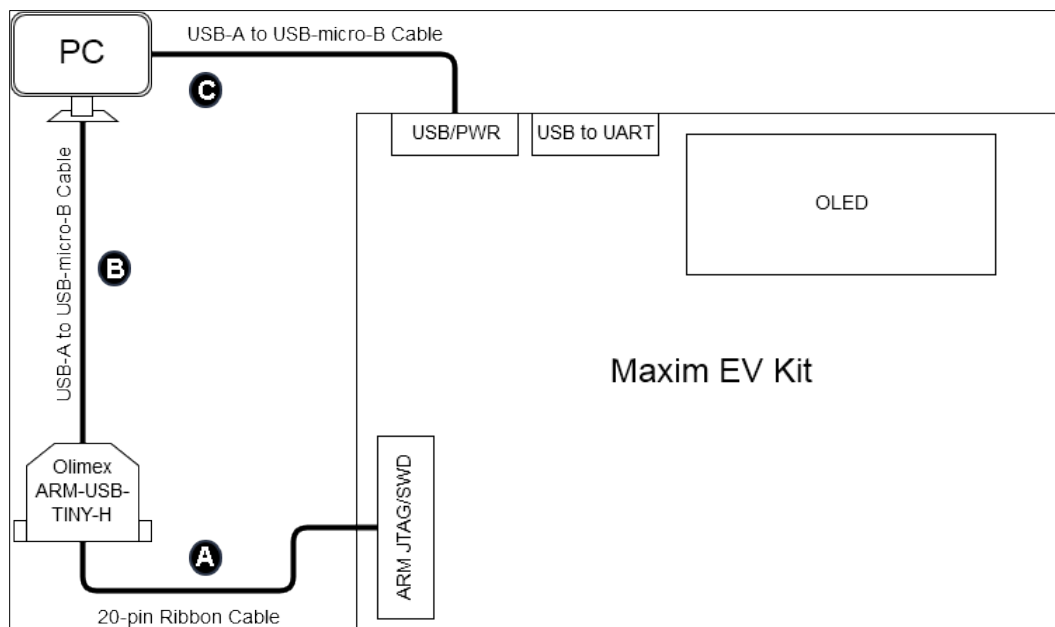
Figure 6. Maxim EV kit connections.
