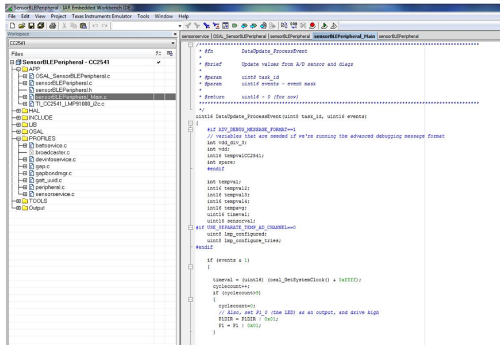
Figure 37. Main Loop
