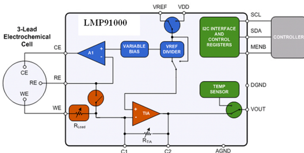
Figure 1. Sensor Design
