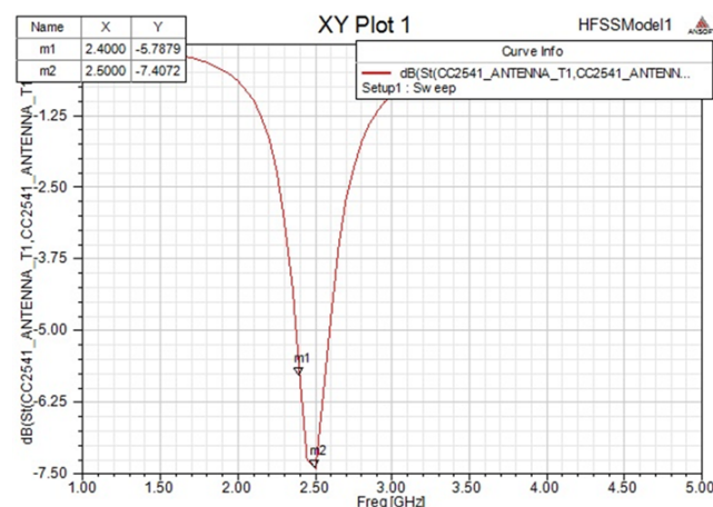
Figure 16. Antenna Simulations Matching With Power Board
