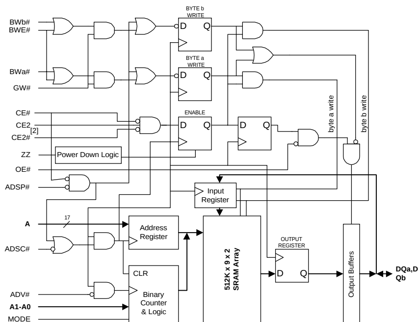
Functional Block Diagram—512K x 18 [1]
