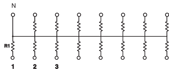
Schematic B Bussed (highest number pin is common)
