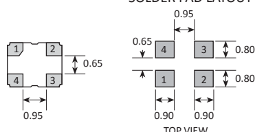
SOLDER PAD LAYOUT
