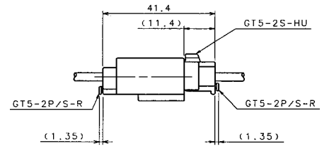
◆ Diagram of Mated Connector in Use
