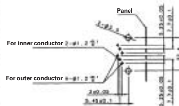
◆ Recommended Board Mounting Pattern
