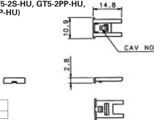
◆ Keying Configurations
