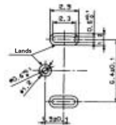
◆ Board Termination Pattern
