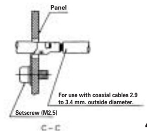
Attachment Diagram
