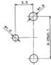
◆ Board Termination Pattern
