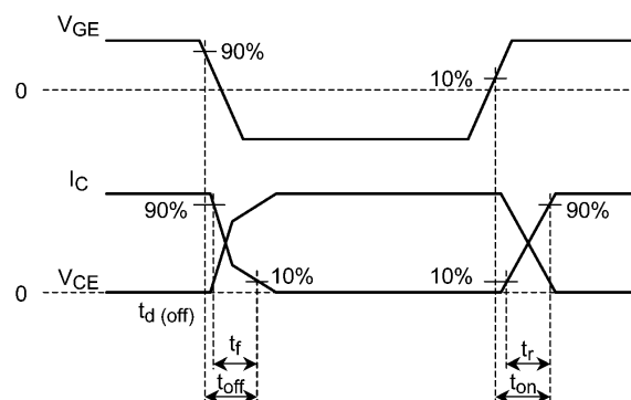
Fig. 6.2.2 Timing Chart of Switching Time
