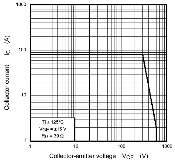
Fig. 8.9 Reverse Bias SOA (Guaranteed Maximum)
