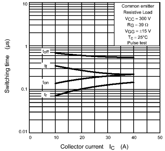
Fig. 8.7 Switching Time - I_C
