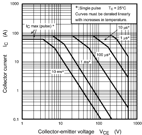
Fig. 8.8 Safe Operating Area (Guaranteed Maximum)
