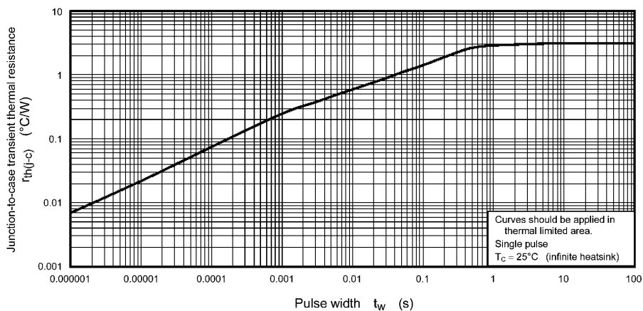
Fig. 8.10 r_{th(j-c)} - t_w (Guaranteed Maximum)
