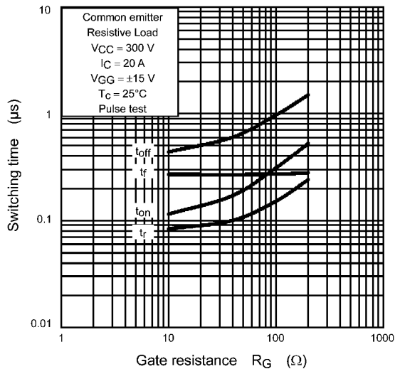
Fig. 8.6 Switching Time - R_G
