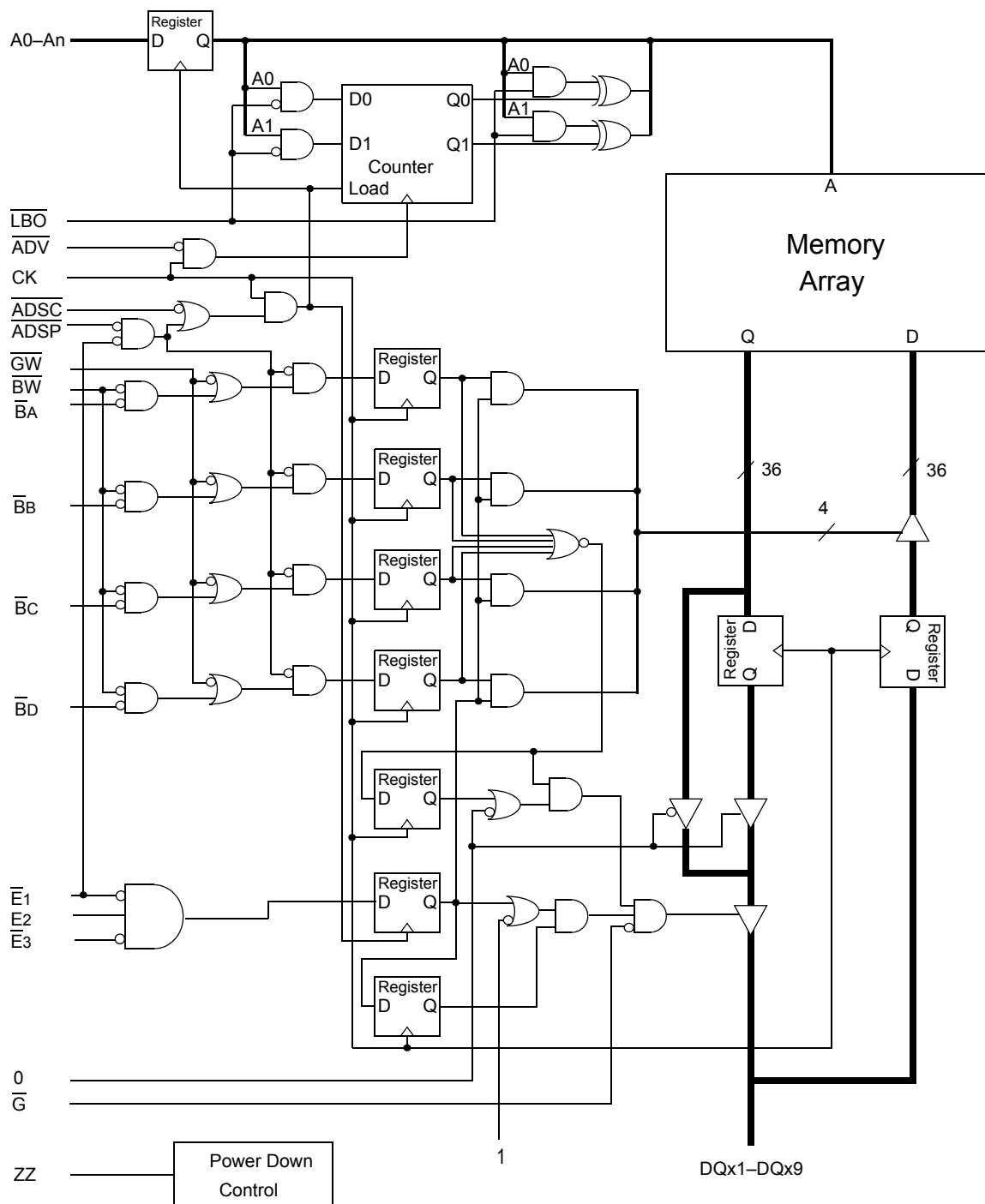
GS8160FxxBT-xxxV Block Diagram
