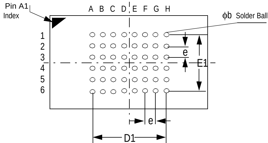
Bottom View
