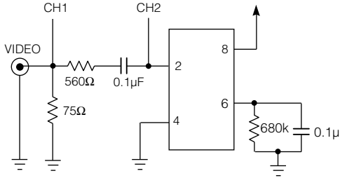
Test Circuit 3
