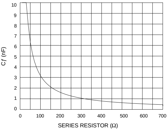
Fig. 24 C_f vs Series Resistor
