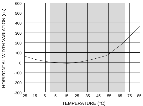
Fig. 12 Horizontal Width Variation vs Temperature
