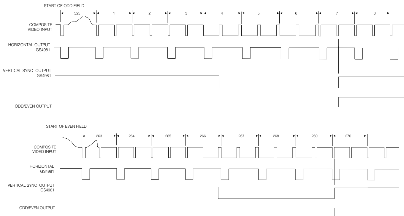
Fig. 28 Timing Diagram
