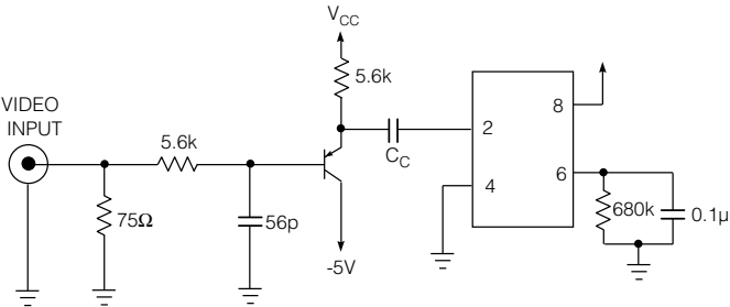
Fig. 26 Typical NTSC Application Circuit
