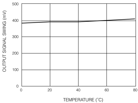
Fig. 18 Output Signal Swing, p-p, Differential
