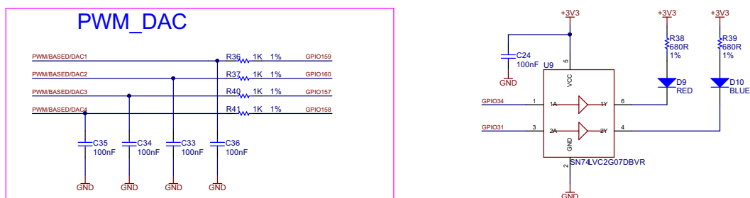
Figure 6. P05_PWM-DAC
