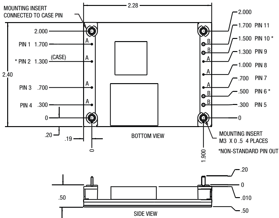
Pin Configuration —Bottom View
