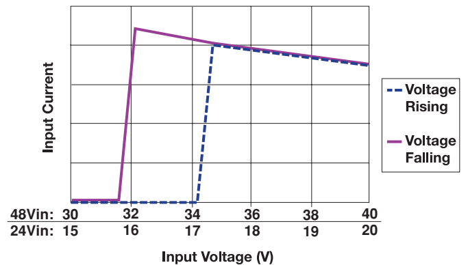
Undervoltage Lockout
