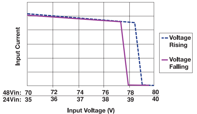
Overvoltage Lockout
