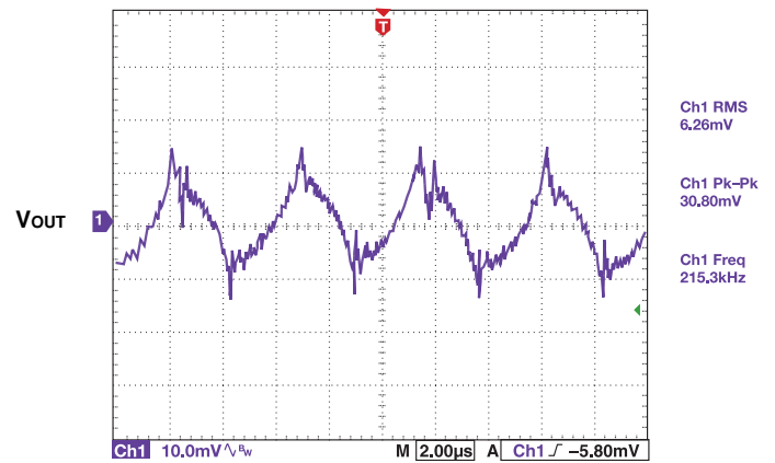
Voltage Ripple
