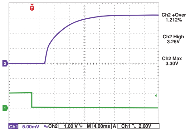
Start-up Waveform
