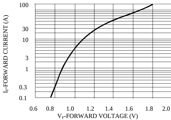
Fig. 5-TYPICAL FORWARD CHARACTERISTICS
