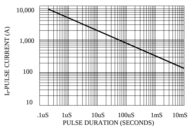
Fig. 6-FORWARD PULSE CURRENT, PULSE
