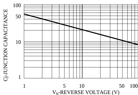
Fig. 4-TYPICAL JUNCTION CAPACITANCE
