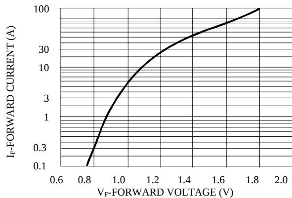
Fig. 5-TYPICAL FORWARD CHARACTERISTICS
