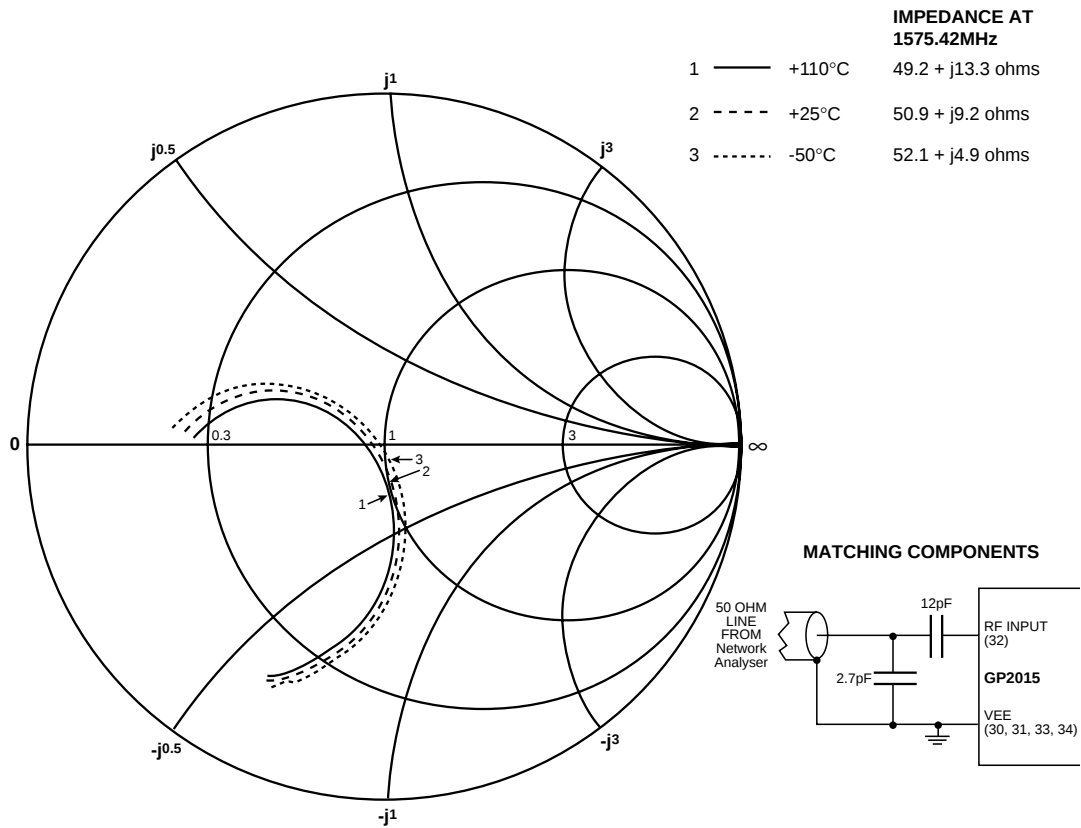
Fig. 28 Typical Matched RF I/P Impedance between 1000MHz and 2000MHz RF I/P level @ -40dBm
