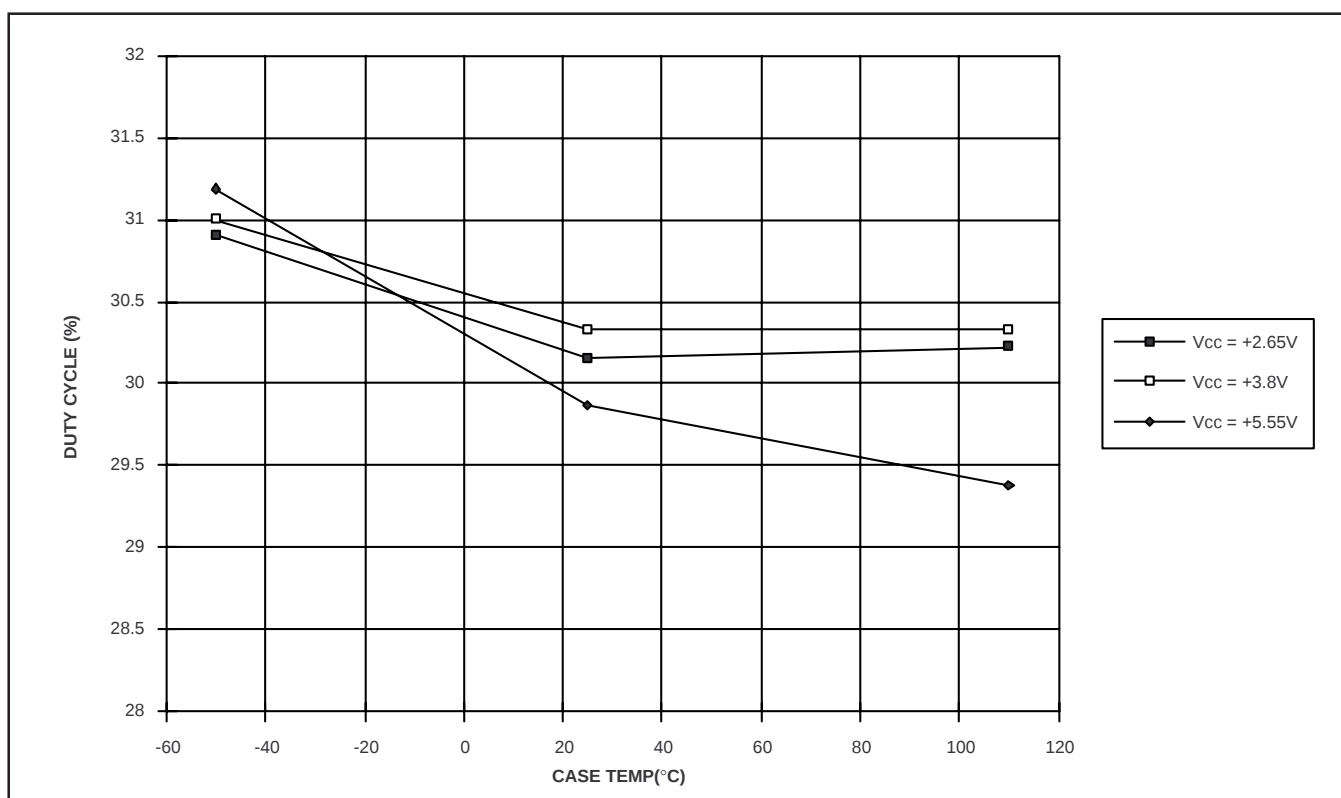
Fig. 25 Duty-cycle of MAG digital output (pin 14), sampled at 5.71MHz in a typical application circuit - RF I/P signal = 1575.42MHz CW, -85dBm - equivalent to 26dB excess noise from a typical GPS antenna
