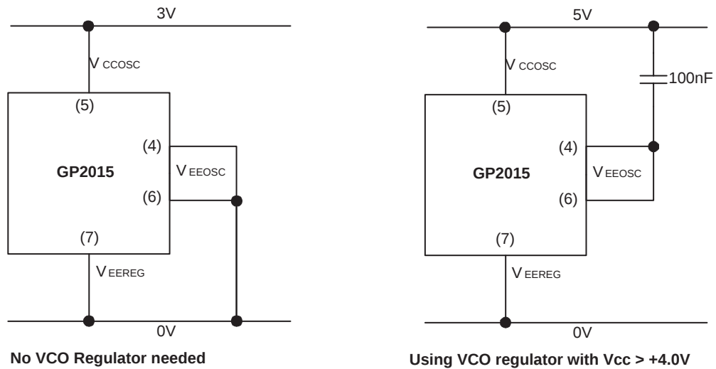
Fig. 7 VCO power-supply connections
