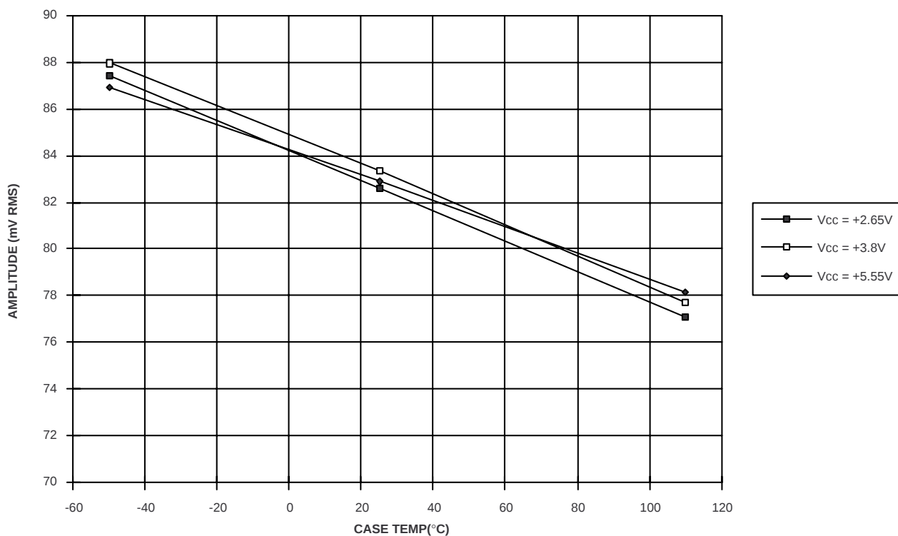
Fig. 27 Amplitude of IFOUT (pin 1) at 4.3MHz ( \pm 1.0 MHz) in a typical application circuit - RF I/P signal = 1575.42MHz CW, -85dBm - equivalent to 26dB excess noise from a typical GPS antenna
