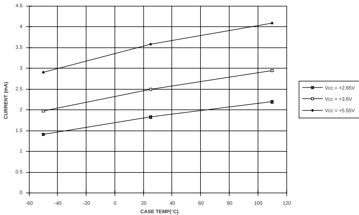
Fig. 11 Supply Current - Digital interface - power-down mode
