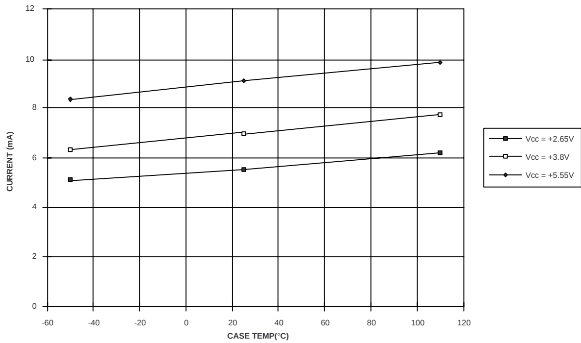
Fig. 10 Supply Current - Digital interface - normal mode
