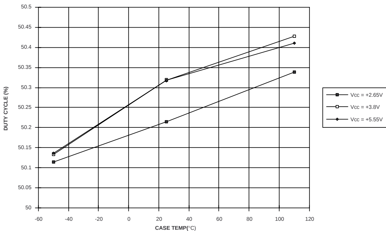
Fig. 26 Duty-cycle of SIGN digital output (pin 15), sampled at 5.71MHz in a typical application circuit - RF I/P signal = 1575.42MHz CW, -85dBm - equivalent to 26dB excess noise from a typical GPS antenna
