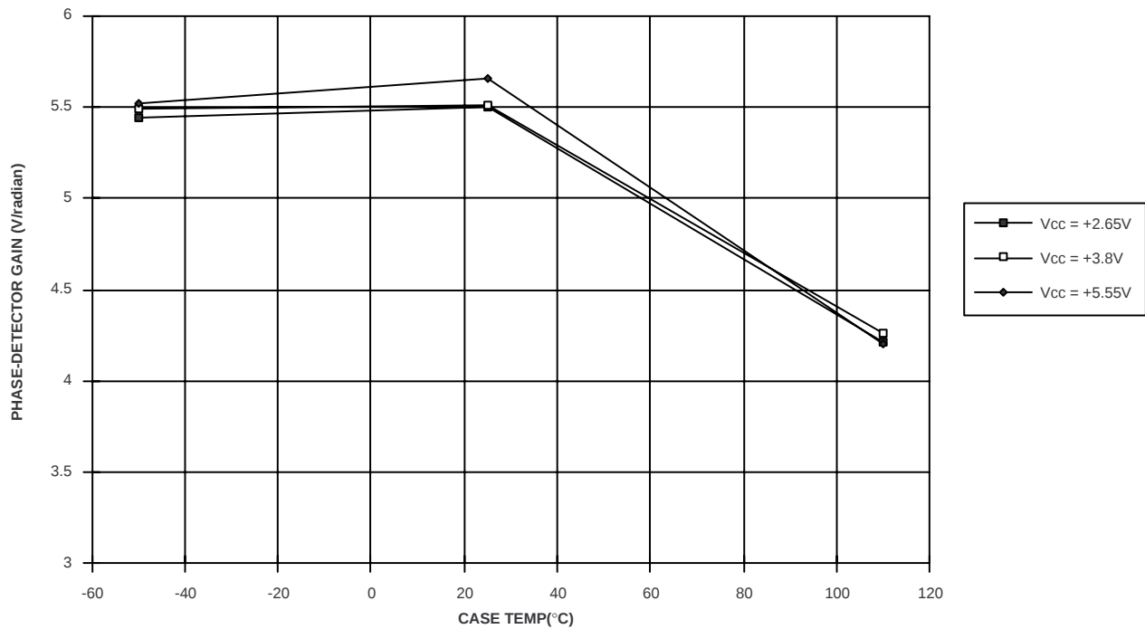
Fig. 14 On-chip Phase-locked-loop Synthesiser Phase-detector gain
