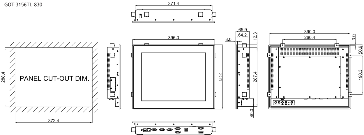
GOT-3156TL-830
