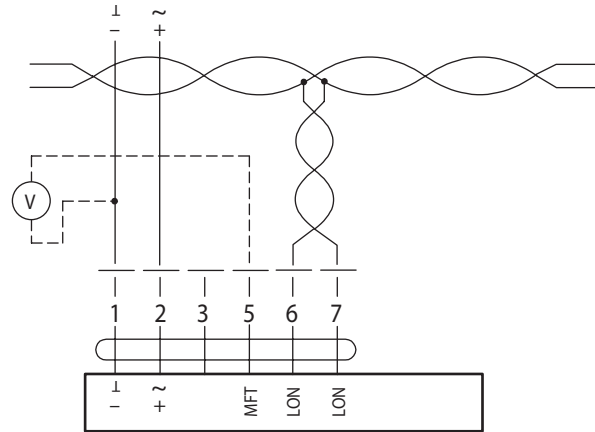
Connection without Sensor
