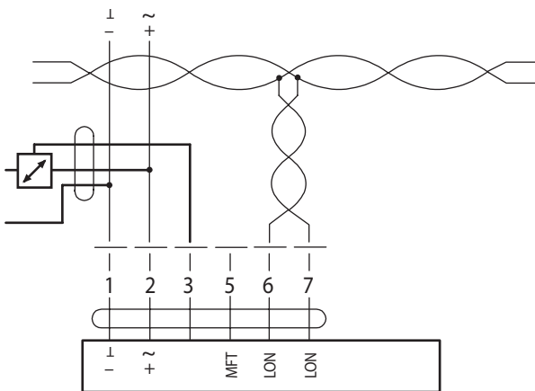
Connection with Active Sensor, e.g. 0... 10 V @ 0...50 C
