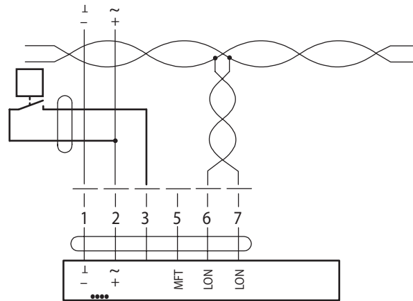
Connection with Switching Contact, e.g. p-monitor
