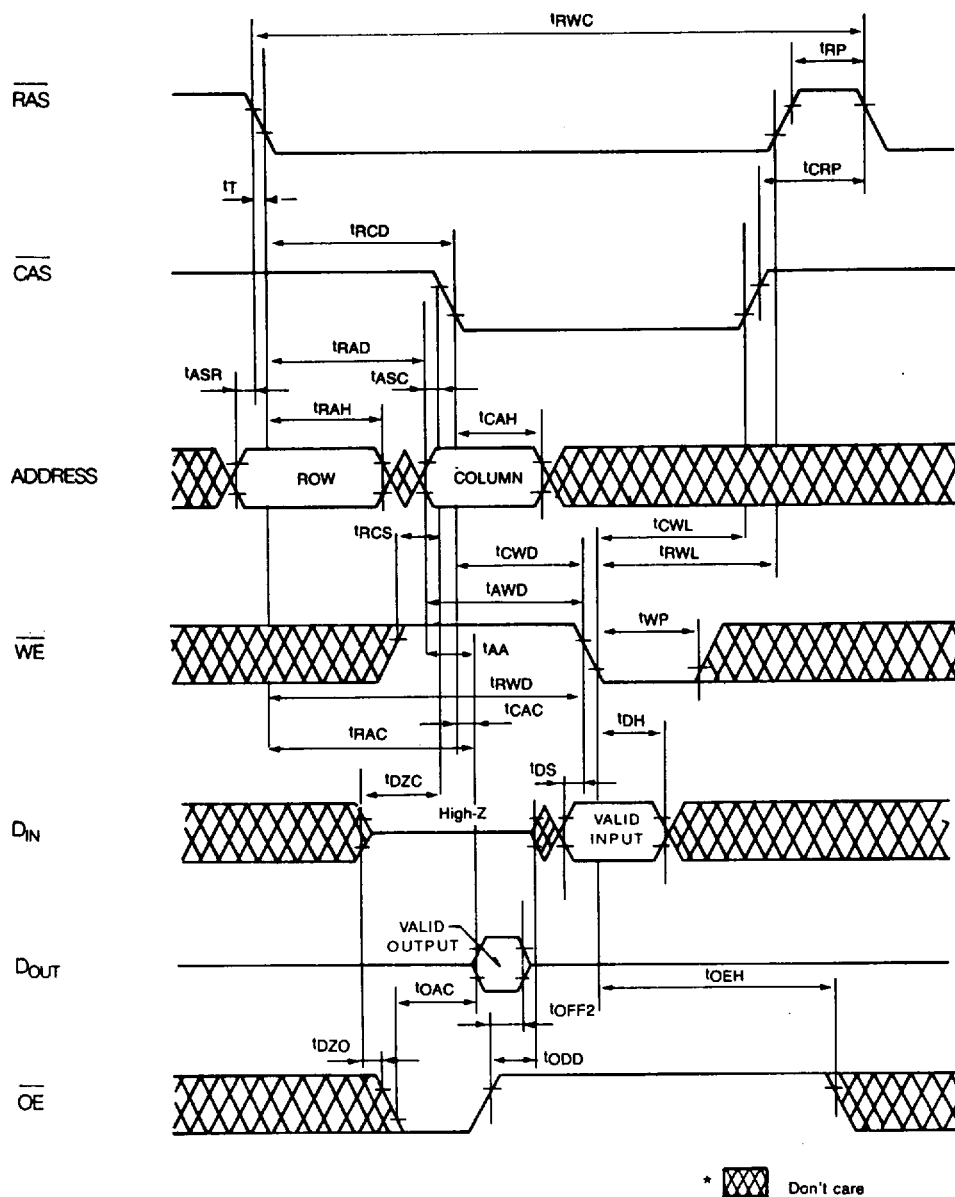
FIGURE 4. READ-MODIFY-WRITE CYCLE
