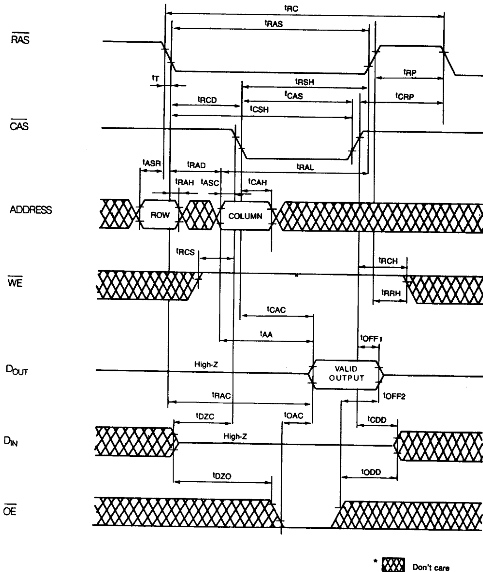
FIGURE 1. READ CYCLE
