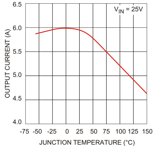
Figure 3. Current Limit
