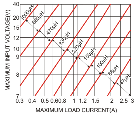
Figure 16. GM7130 -5.0
