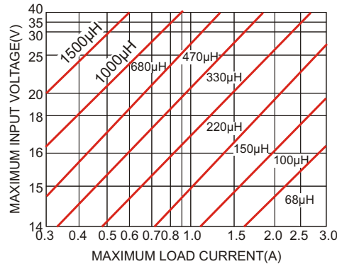
Figure 15. GM7130 - 12
