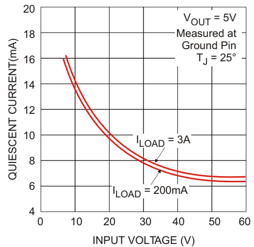
Figure 5. Quiescent Current
