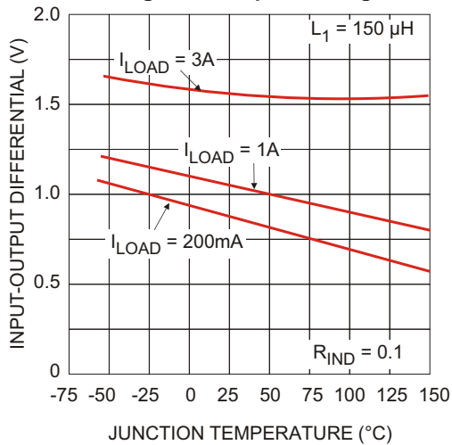
Figure 4. Dropout Voltage
