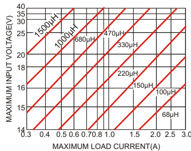
Figure 15. GM7130 -12
