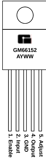
TO-220-5
